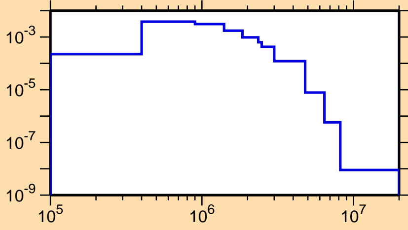
\sigma vs. E for ^{172}\text{Re}(n,n_3)
