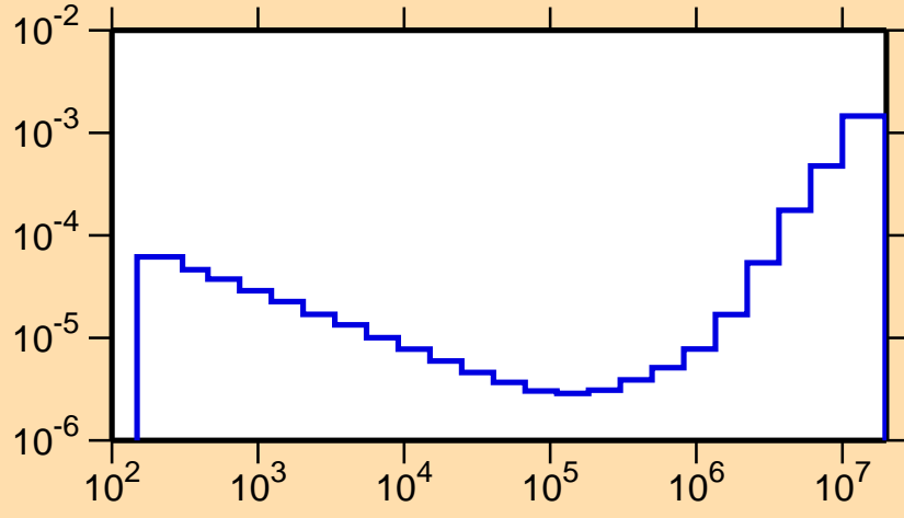
\sigma vs. E for ^{172}\text{Re}(n,p\alpha)
