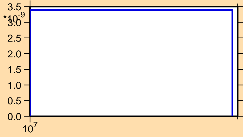
\sigma vs. E for ^{172}\text{Re}(n,\text{pt})
