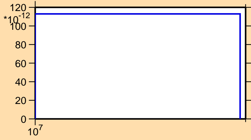
\sigma vs. E for ^{172}\text{Re}(n,3n\alpha)
