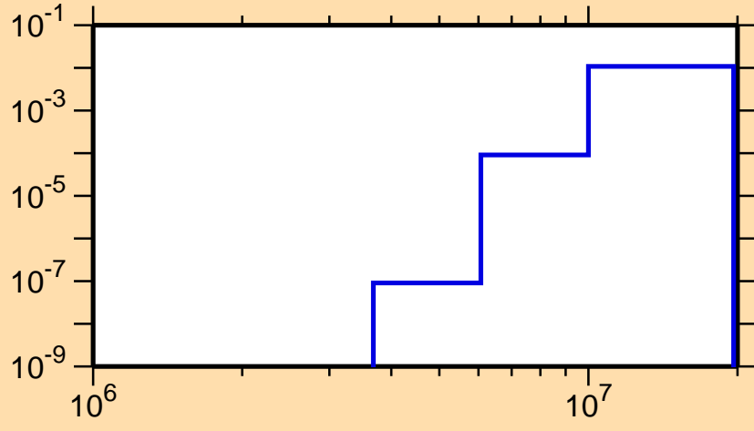
\sigma vs. E for ^{172}\text{Re}(n,d)
