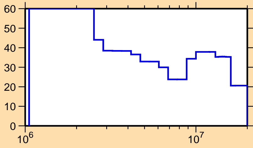
\Delta\sigma/\sigma vs. E for ^{173}\text{Re}(n,n\text{cont.})
