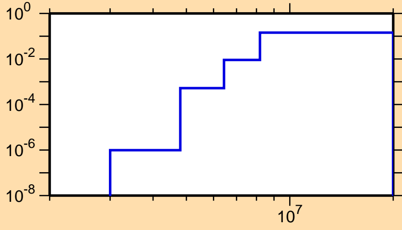
\sigma vs. E for ^{173}\text{Re}(n,np)
