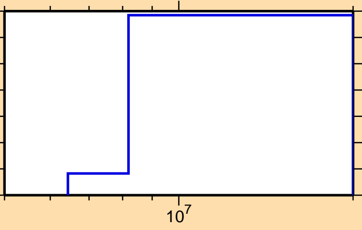
\sigma vs. E for ^{173}\text{Re}(\text{mt117})
