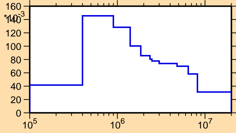
\sigma vs. E for ^{173}\text{Re}(n,n_2)
