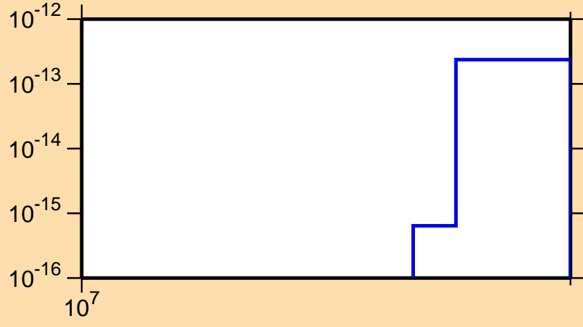
\sigma vs. E for ^{174}\text{Re}(n,3n\alpha)
