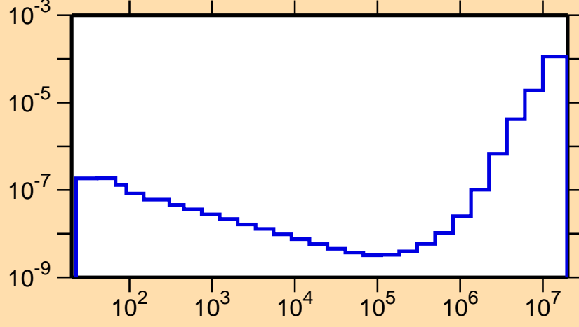
\sigma vs. E for ^{174}\text{Re}(n,p\alpha)
