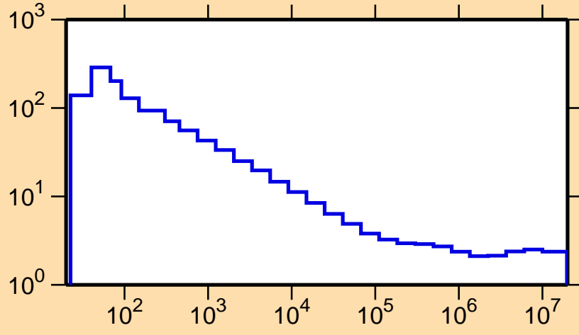
\sigma vs. E for ^{174}\text{Re}(n,\text{nonel.})
