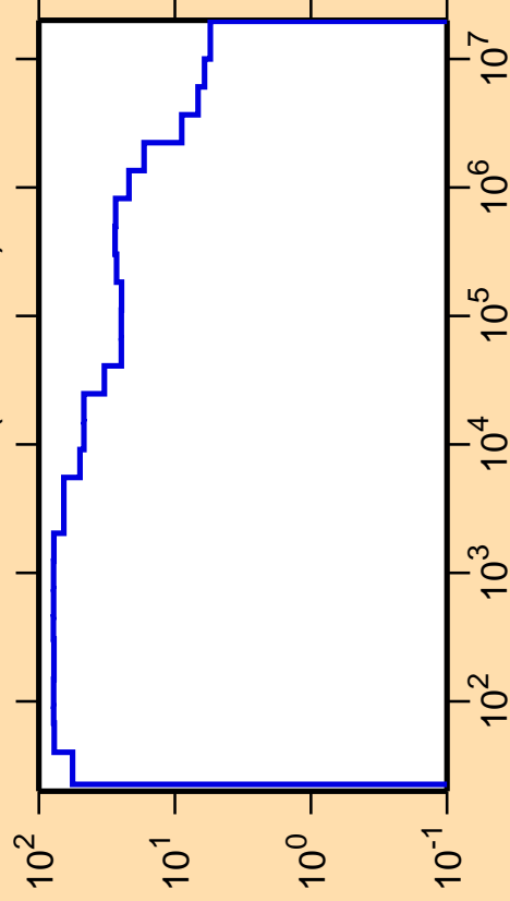
\Delta\sigma/\sigma vs. E for ^{174}\text{Re}(n,\text{nonel.})
