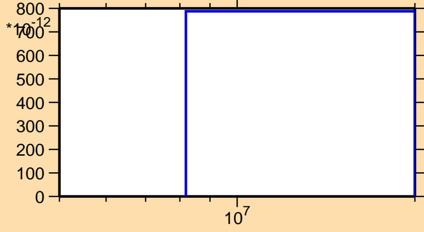
\sigma vs. E for ^{174}\text{Re}(n,\text{pd})
