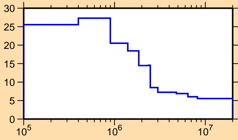
\Delta\sigma/\sigma vs. E for ^{174}\text{Re}(n,\text{nonel.})
