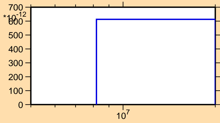
\sigma vs. E for ^{174}\text{Re}(n,nt)
