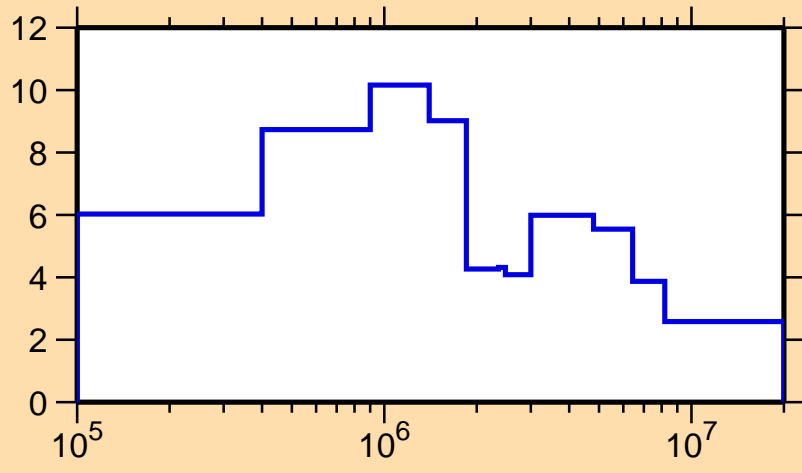
\Delta\sigma/\sigma vs. E for ^{174}\text{Re}(n,\text{tot.})
