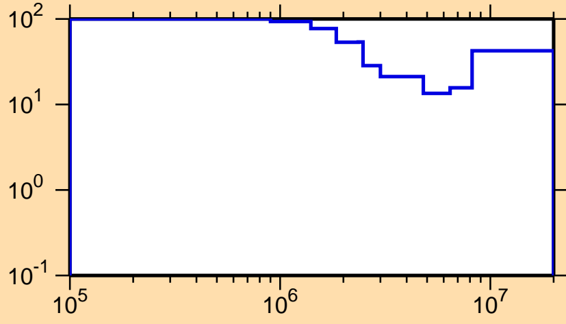
\Delta\sigma/\sigma vs. E for ^{174}\text{Re}(n,n\text{cont.})
