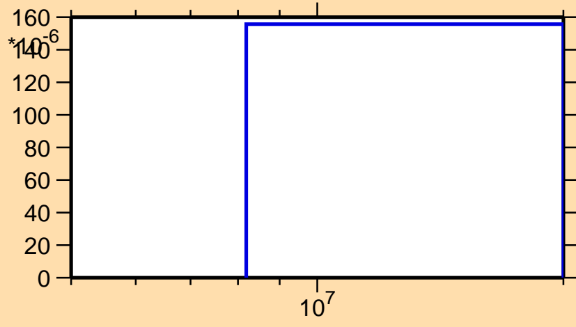
\sigma vs. E for ^{174}\text{Re}(n,2n\alpha)
