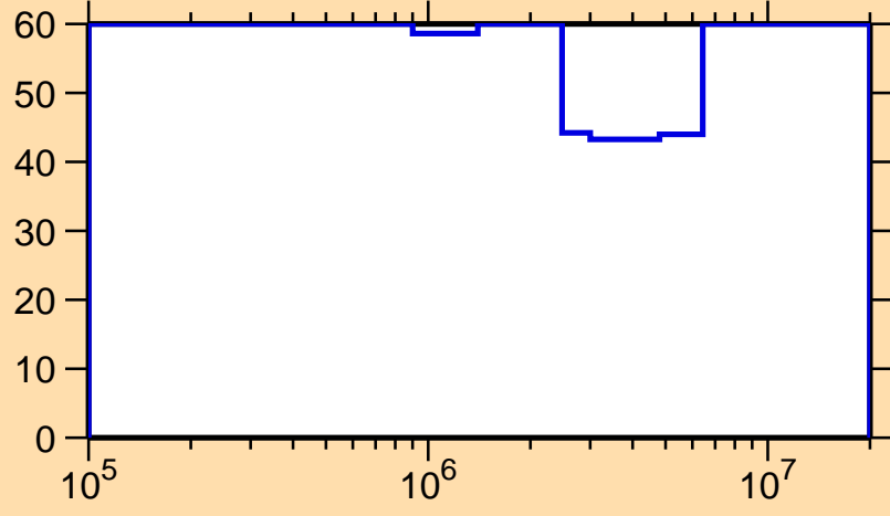
\Delta\sigma/\sigma vs. E for ^{174}\text{Re}(n,n_1)
