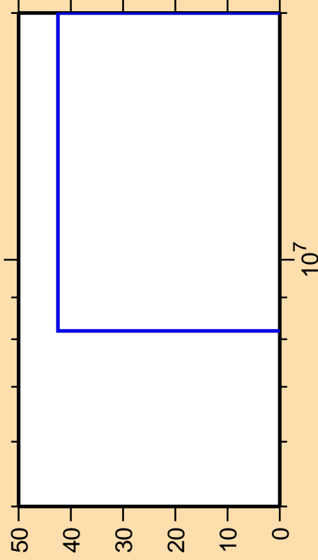
\Delta\sigma/\sigma vs. E for ^{174}\text{Re}(n,n\text{cont.})
