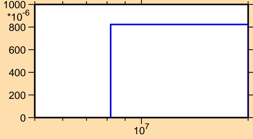
\sigma vs. E for ^{174}\text{Re}(n,2np)
