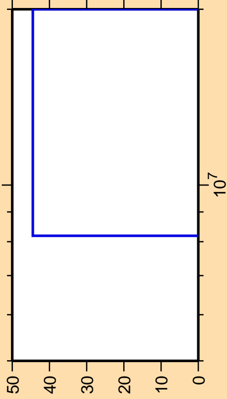
\Delta\sigma/\sigma vs. E for ^{174}\text{Re}(n,p)
