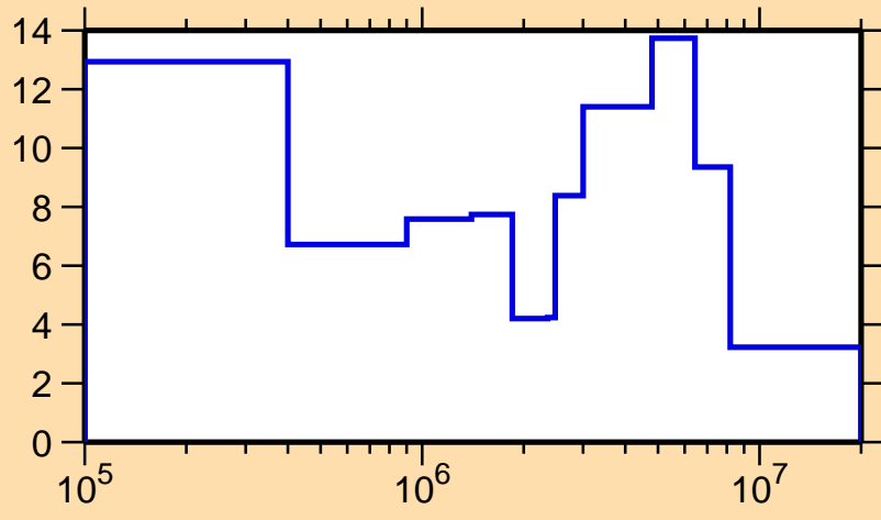
\Delta\sigma/\sigma vs. E for ^{174}\text{Re}(n,\text{el.})
