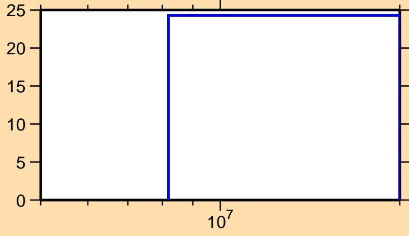
\Delta\sigma/\sigma vs. E for ^{174}\text{Re}(n,2n)
