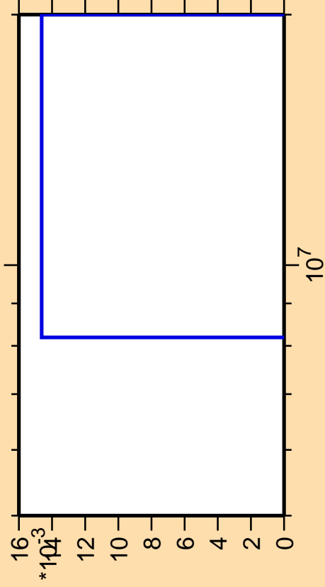
\Delta\sigma/\sigma vs. E for ^{174}\text{Re}(n,3n\alpha)
