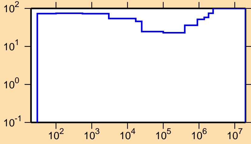
\Delta\sigma/\sigma vs. E for ^{174}\text{Re}(n,\gamma)
