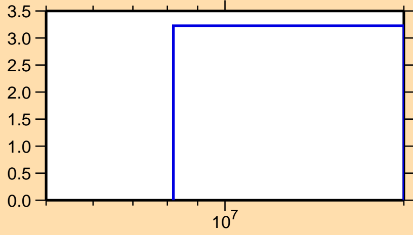
\Delta\sigma/\sigma vs. E for ^{174}\text{Re}(n,\text{el.})
