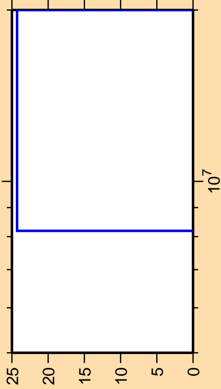
\Delta\sigma/\sigma vs. E for ^{174}\text{Re}(n,2n)
