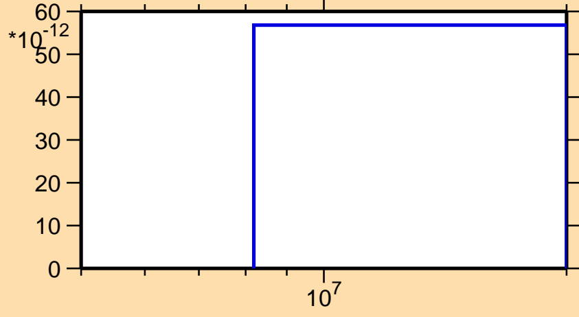
\sigma vs. E for ^{174}\text{Re}(n,\text{pt})
