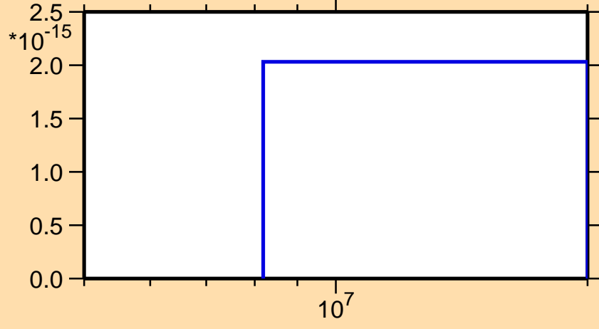
\sigma vs. E for ^{174}\text{Re}(n,3n\alpha)
