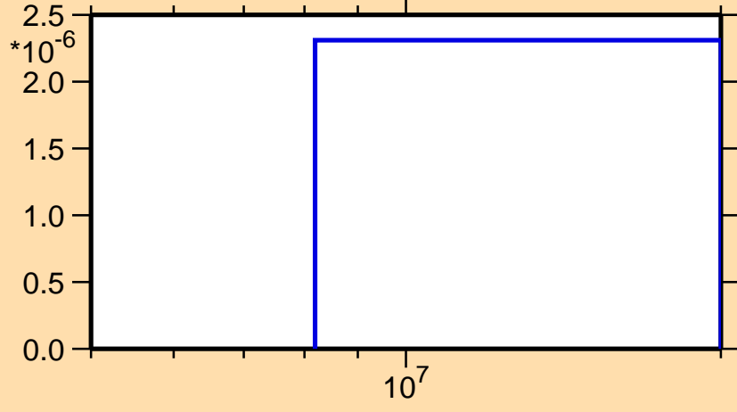
\sigma vs. E for ^{174}\text{Re}(n,3n)
