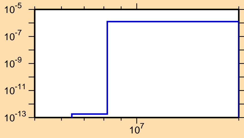
\sigma vs. E for ^{174}\text{Re}(n,\text{He3})
