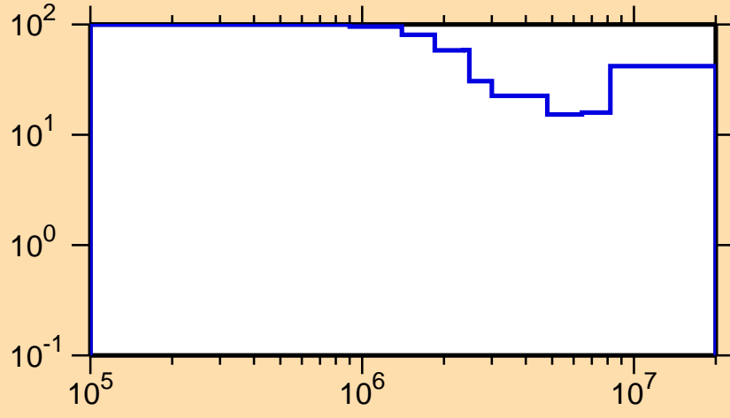
\Delta\sigma/\sigma vs. E for ^{174}\text{Re}(n,\text{inel.})
