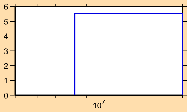
\Delta\sigma/\sigma vs. E for ^{174}\text{Re}(n,\text{nonel.})
