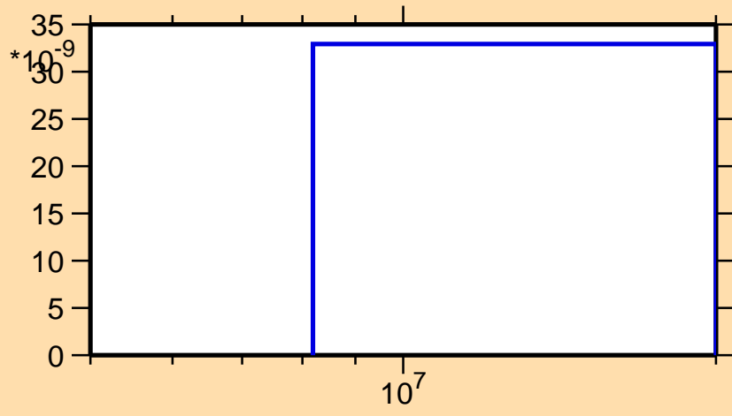
\sigma vs. E for ^{174}\text{Re}(\text{mt117})
