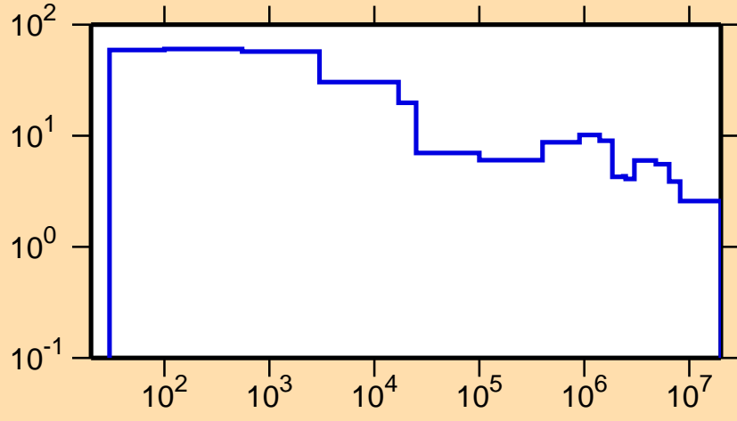
\Delta\sigma/\sigma vs. E for ^{174}\text{Re}(n,\text{tot.})
