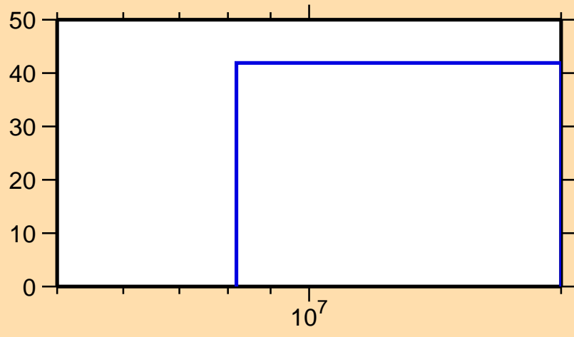
\Delta\sigma/\sigma vs. E for ^{174}\text{Re}(n,\text{inel.})
