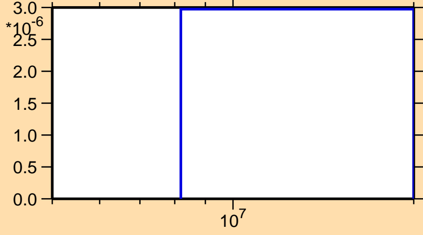
\sigma vs. E for ^{174}\text{Re}(n,\text{nd})
