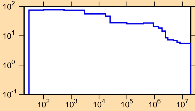
\Delta\sigma/\sigma vs. E for ^{174}\text{Re}(n,\text{nonel.})
