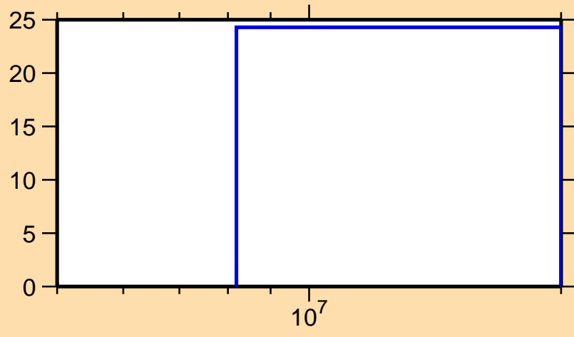
\Delta\sigma/\sigma vs. E for ^{174}\text{Re}(n,2n)
