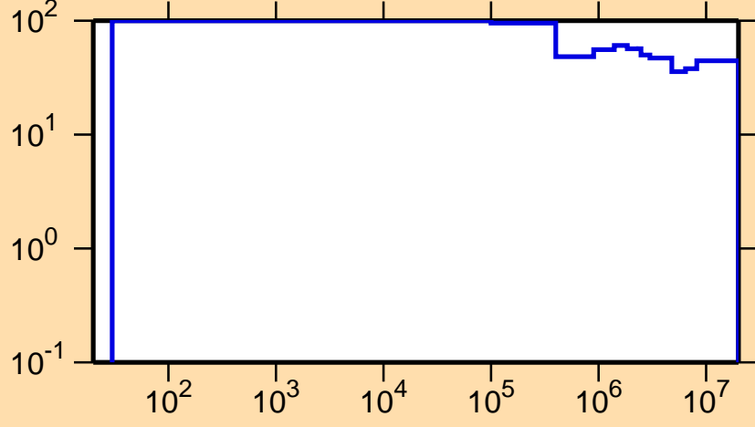
\Delta\sigma/\sigma vs. E for ^{174}\text{Re}(n,p)
