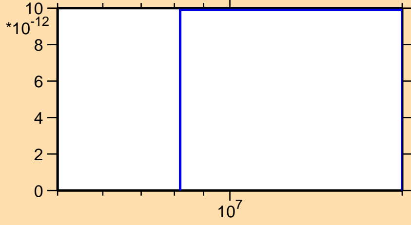
\sigma vs. E for ^{174}\text{Re}(\text{mt } 34)
