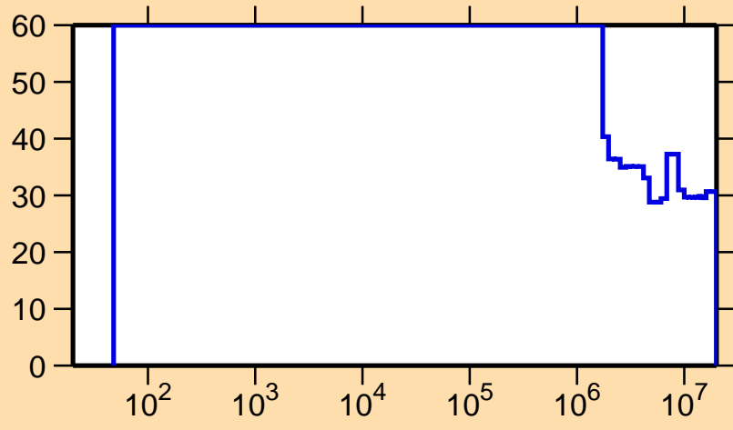
\Delta\sigma/\sigma vs. E for ^{175}\text{Re}(n,p)
