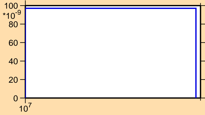
\sigma vs. E for ^{175}\text{Re}(n,\text{nd})
