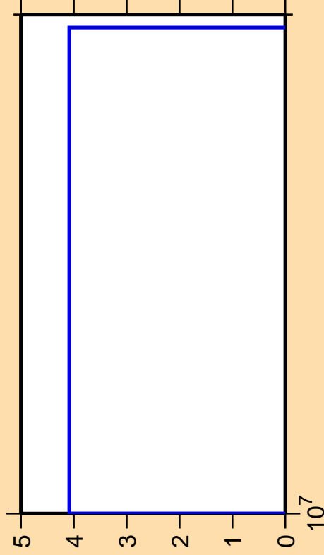
\Delta\sigma/\sigma vs. E for ^{175}\text{Re}(n,3n\alpha)
