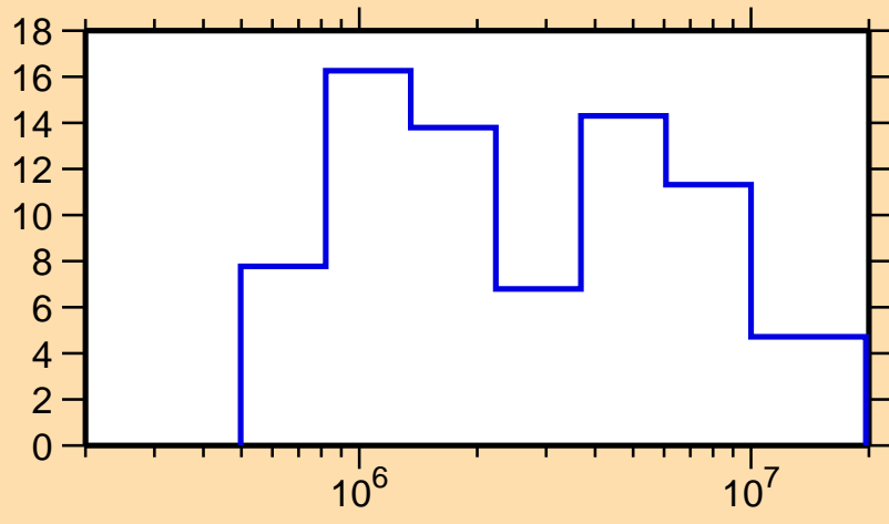
\Delta\sigma/\sigma vs. E for ^{175}\text{Re}(n, el.)
