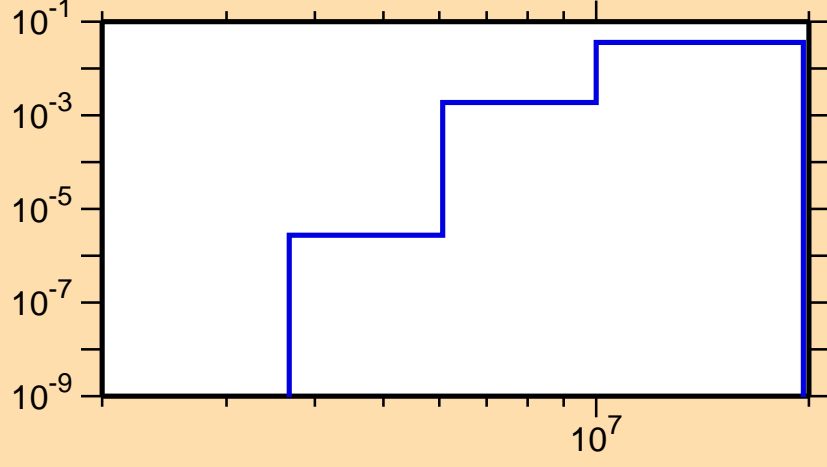
\sigma vs. E for ^{175}\text{Re}(n,np)
