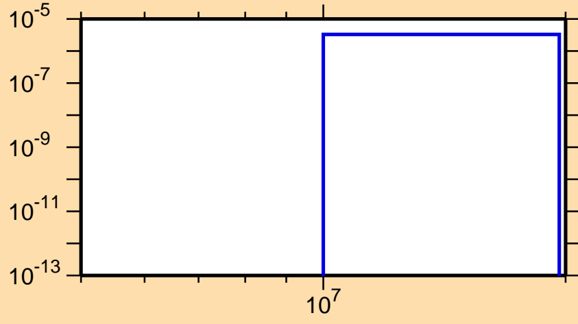
\sigma vs. E for ^{175}\text{Re}(n,2n\alpha)
