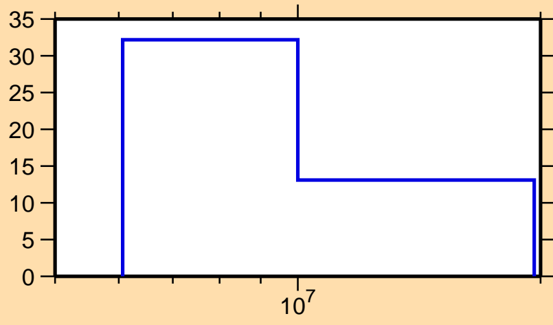
\Delta\sigma/\sigma vs. E for ^{175}\text{Re}(n,2n)
