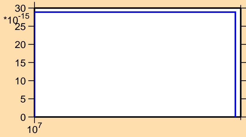
\sigma vs. E for ^{175}\text{Re}(\text{mt } 34)
