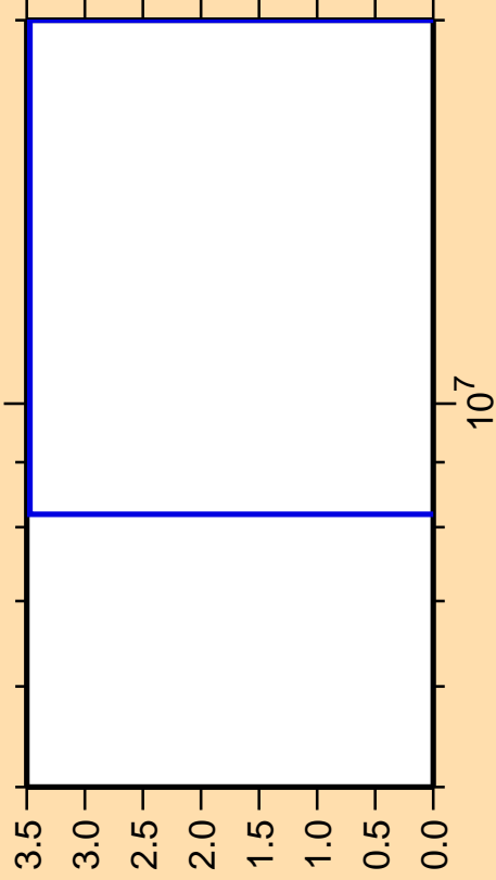
\Delta\sigma/\sigma vs. E for ^{175}\text{Re}(n,3n\alpha)
