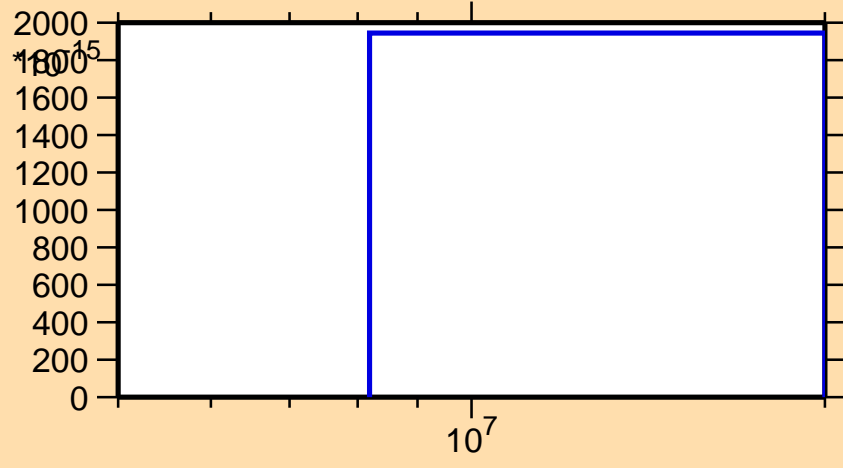
\sigma vs. E for ^{175}\text{Re}(n,3n\alpha)
