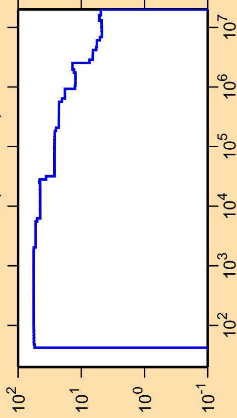
\Delta\sigma/\sigma vs. E for ^{176}\text{Re}(n,\text{nonel.})
