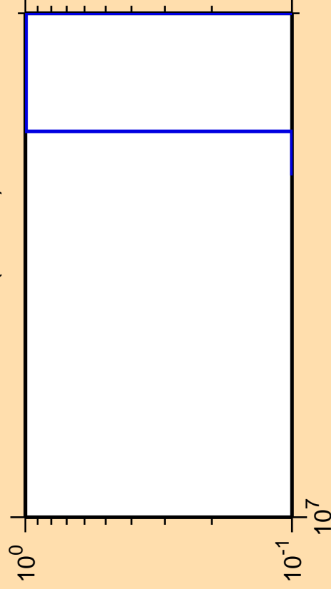
\Delta\sigma/\sigma vs. E for ^{176}\text{Re}(n,3n\alpha)
