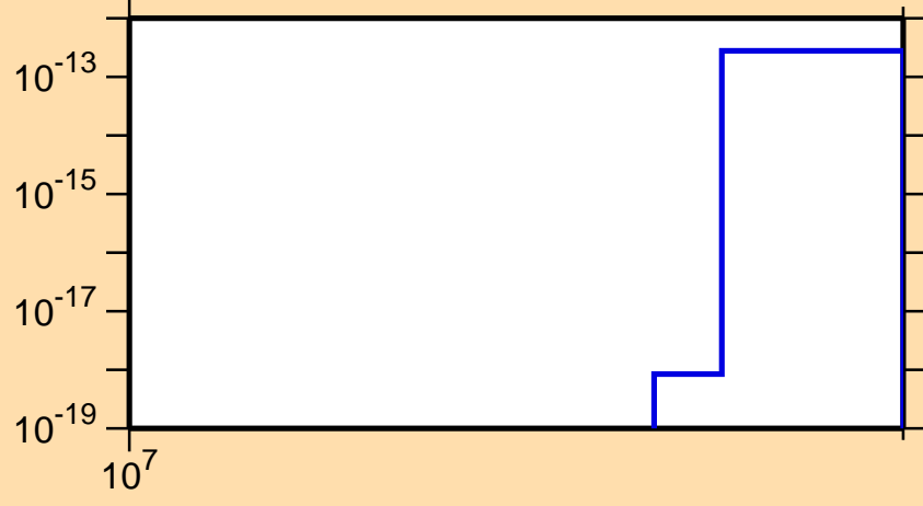
\sigma vs. E for ^{176}\text{Re}(n,3n\alpha)
