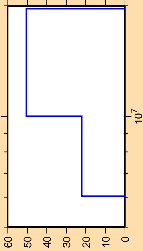
\Delta\sigma/\sigma vs. E for ^{176}\text{Re}(n,n_1)
