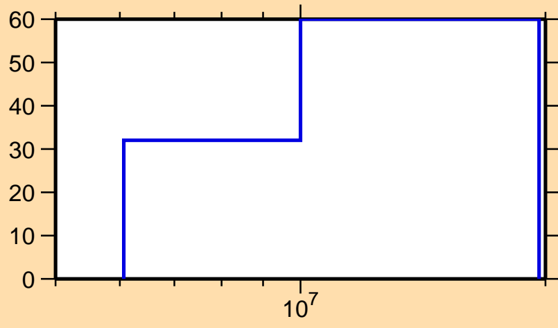
\Delta\sigma/\sigma vs. E for ^{176}\text{Re}(n,\text{inel.})
