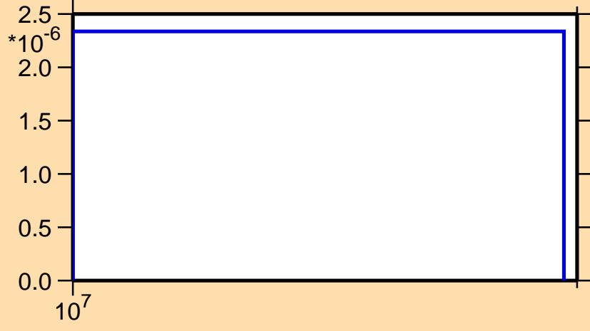
\sigma vs. E for ^{176}\text{Re}(n,\text{nd})
