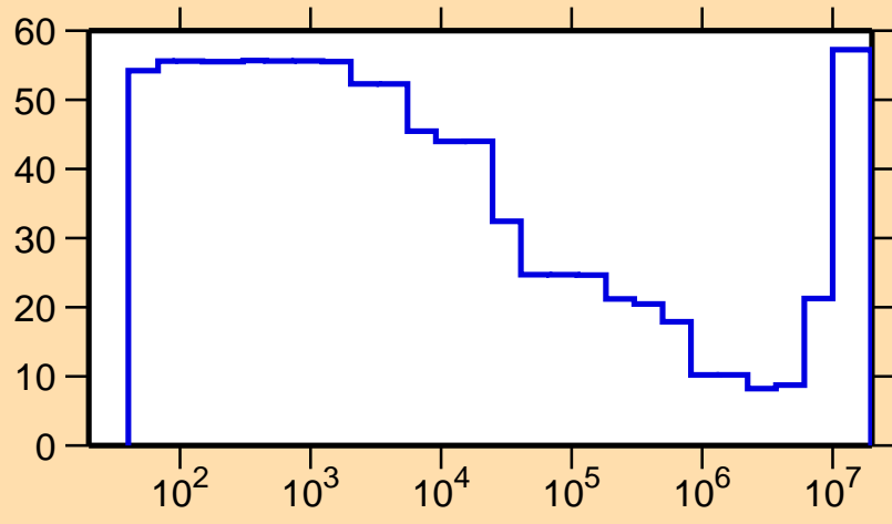
\Delta\sigma/\sigma vs. E for ^{176}\text{Re}(n,\gamma)
