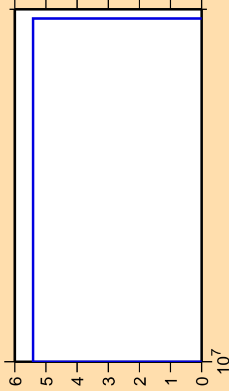
\Delta\sigma/\sigma vs. E for ^{176}\text{Re}(\text{mt } 34)
