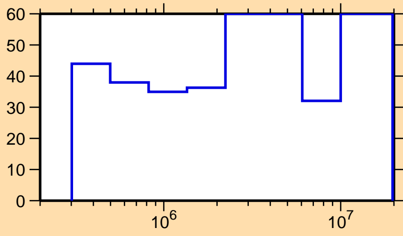
\Delta\sigma/\sigma vs. E for ^{176}\text{Re}(n,n\text{cont.})
