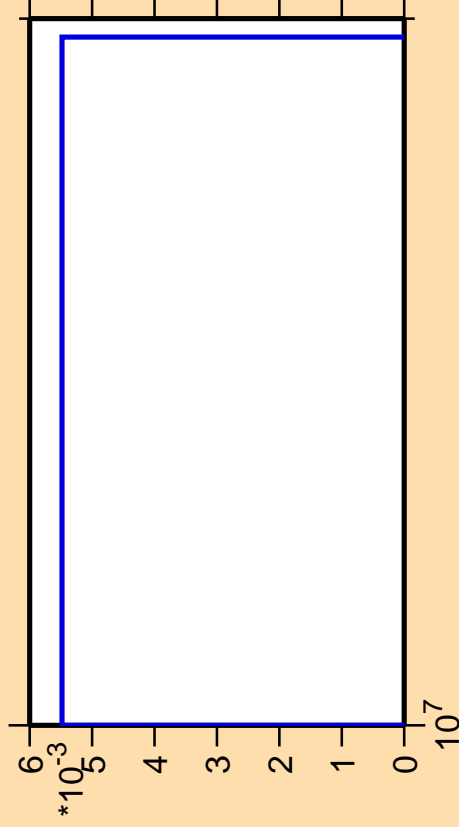
\Delta\sigma/\sigma vs. E for ^{176}\text{Re}(n,3n\alpha)
