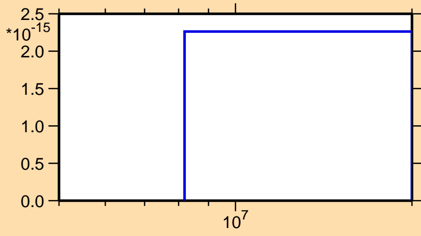
\sigma vs. E for ^{176}\text{Re}(n,3n\alpha)
