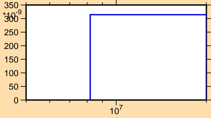
\sigma vs. E for ^{176}\text{Re}(n,\text{He3})
