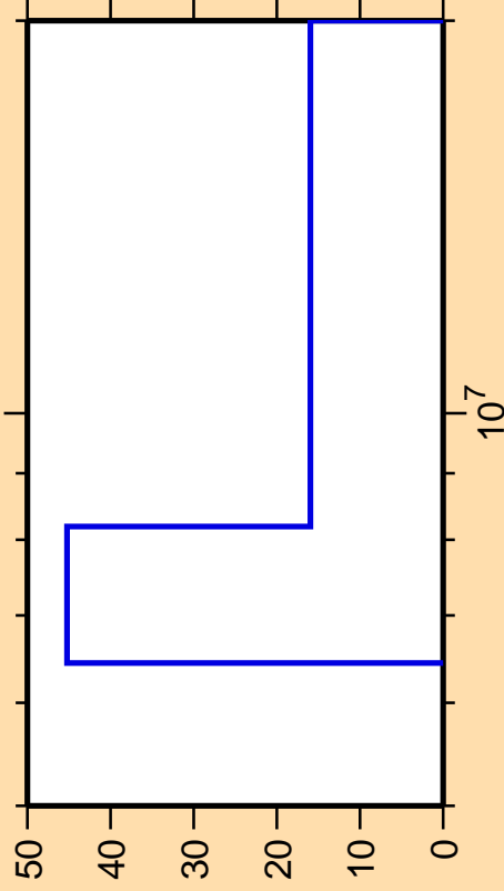
\Delta\sigma/\sigma vs. E for ^{176}\text{Re}(n,2n)
