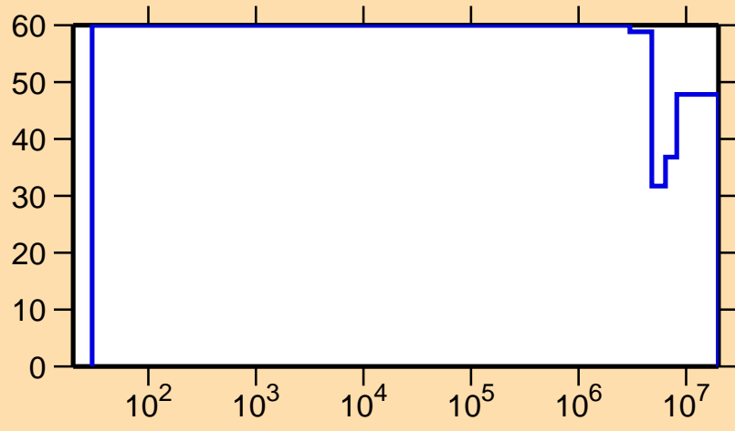
\Delta\sigma/\sigma vs. E for ^{176}\text{Re}(n,p)
