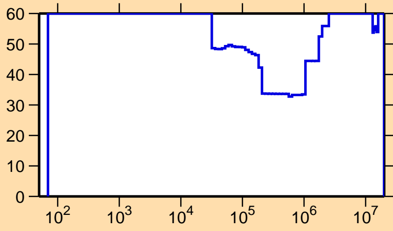
\Delta\sigma/\sigma vs. E for ^{177}\text{Re}(n,\gamma)
