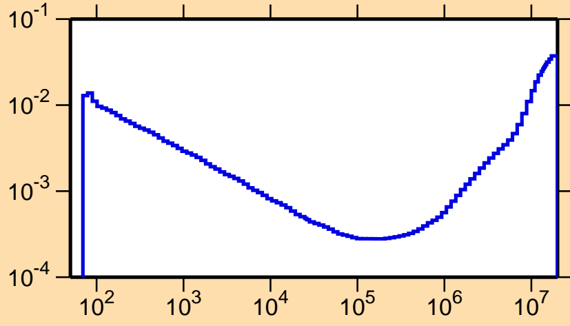
\sigma vs. E for ^{177}\text{Re}(n,p)
