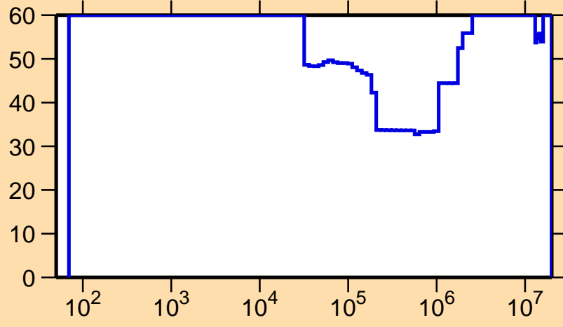
\Delta\sigma/\sigma vs. E for ^{177}\text{Re}(n,\gamma)
