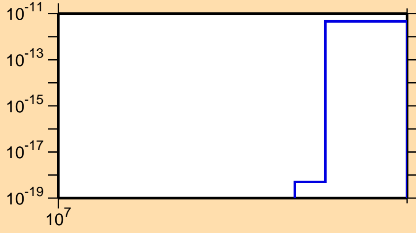
\sigma vs. E for ^{177}\text{Re}(n,3n\alpha)
