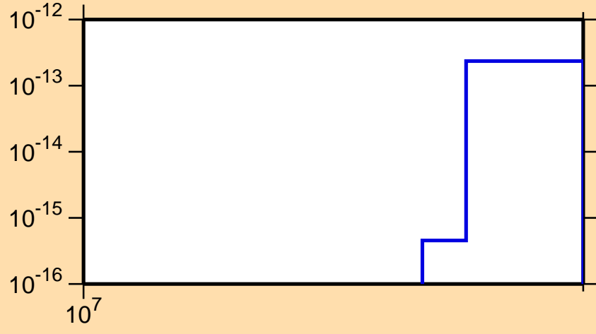
\sigma vs. E for ^{177}\text{Re}(n,\text{pt})
