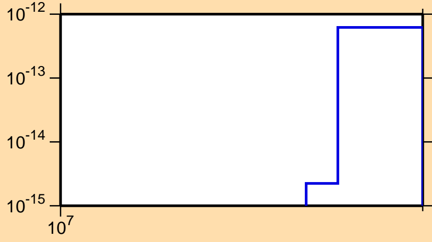
\sigma vs. E for ^{177}\text{Re}(\text{mt } 34)
