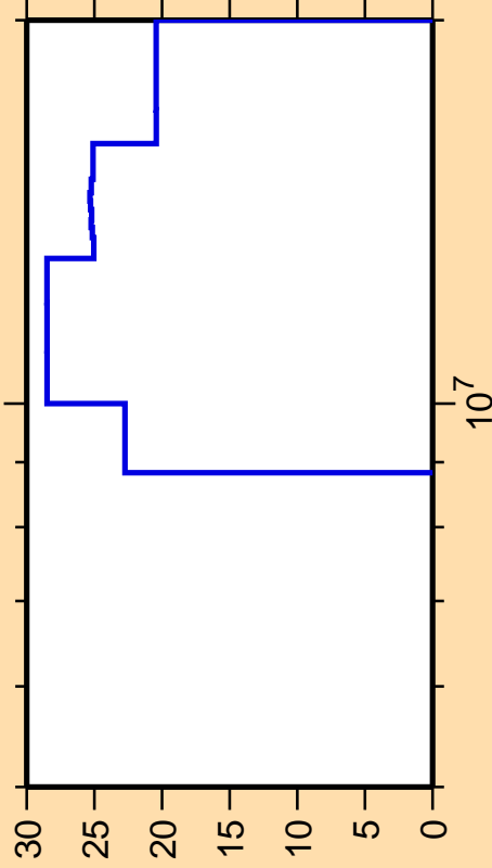
\Delta\sigma/\sigma vs. E for ^{177}\text{Re}(n,n\text{cont.})
