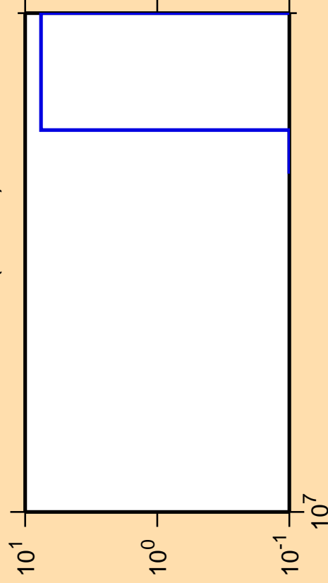
\Delta\sigma/\sigma vs. E for ^{177}\text{Re}(n,3n\alpha)
