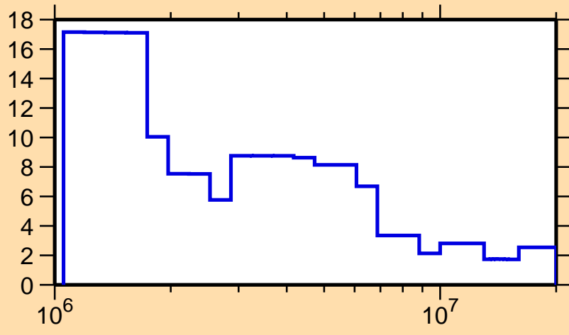
\Delta\sigma/\sigma vs. E for ^{177}\text{Re}(n,\text{tot.})
