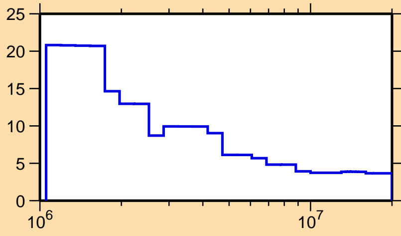
\Delta\sigma/\sigma vs. E for ^{177}\text{Re}(n,n\text{onel.})
