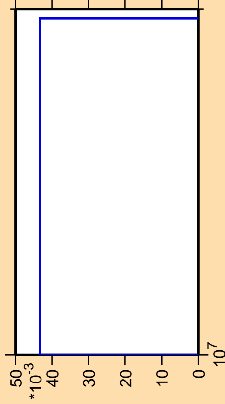
\Delta\sigma/\sigma vs. E for ^{177}\text{Re}(n,3n\alpha)
