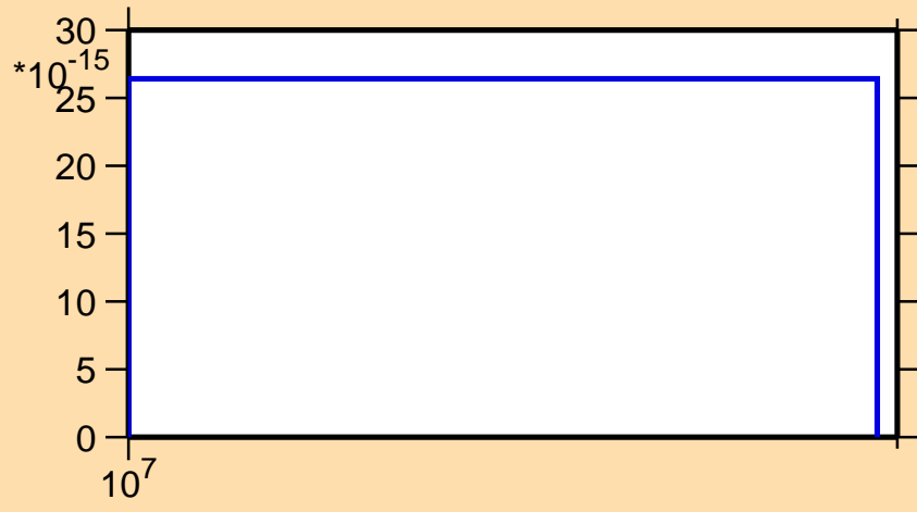
\sigma vs. E for ^{177}\text{Re}(n,3n\alpha)
