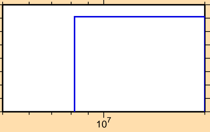
\sigma vs. E for ^{177}\text{Re}(n,pd)
