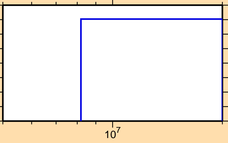
\sigma vs. E for ^{177}\text{Re}(n,\text{He}3)
