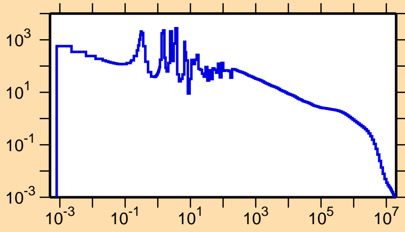
\sigma vs. E for ^{178}\text{Re}(n,\gamma)
