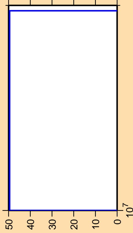
\Delta\sigma/\sigma vs. E for ^{178}\text{Re}(n,3n\alpha)
