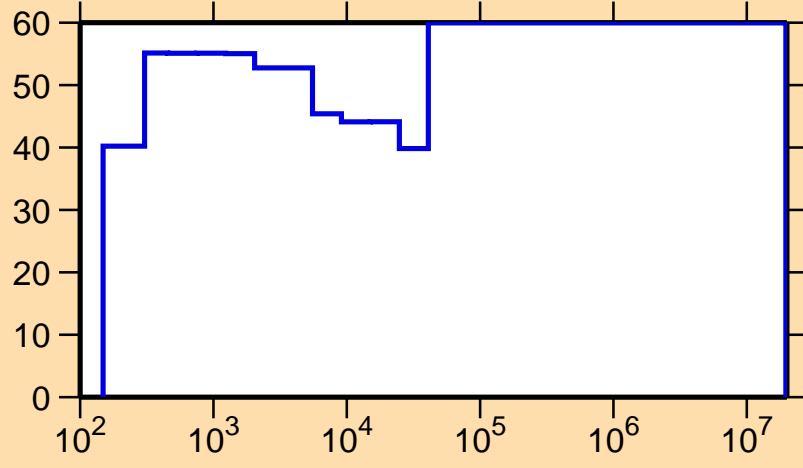
\Delta\sigma/\sigma vs. E for ^{178}\text{Re}(n,\gamma)
