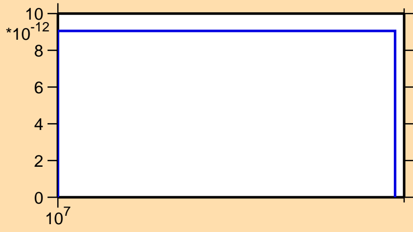
\sigma vs. E for ^{178}\text{Re}(n,3n\alpha)
