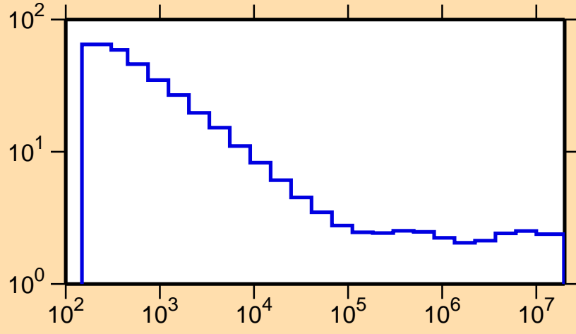
\sigma vs. E for ^{178}\text{Re}(n,\text{nonel.})
