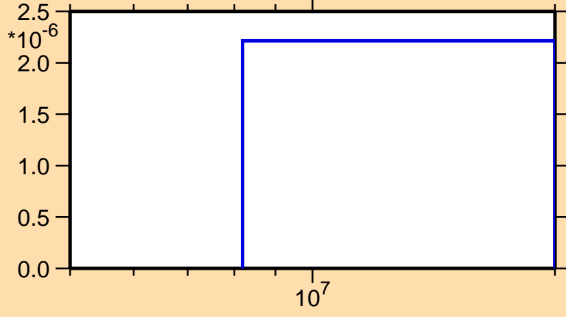
\sigma vs. E for ^{178}\text{Re}(n,\text{nd})
