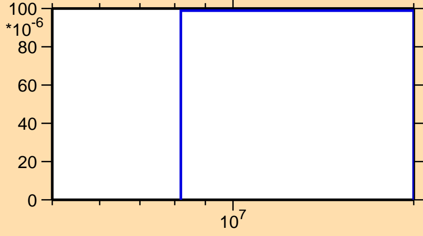
\sigma vs. E for ^{178}\text{Re}(n,3n)
