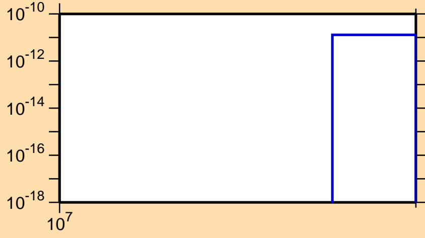
\sigma vs. E for ^{179}\text{Re}(n,3n\alpha)
