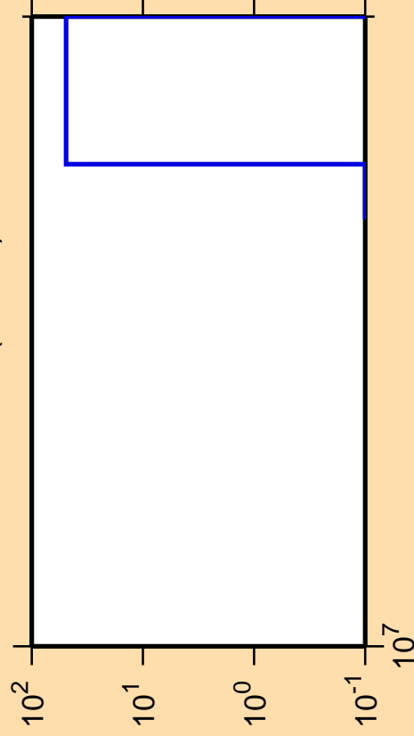
\Delta\sigma/\sigma vs. E for ^{179}\text{Re}(n,3n\alpha)
