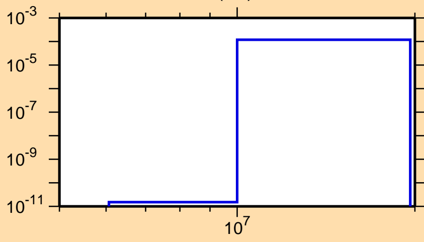
\sigma vs. E for ^{179}\text{Re}(n,t)
