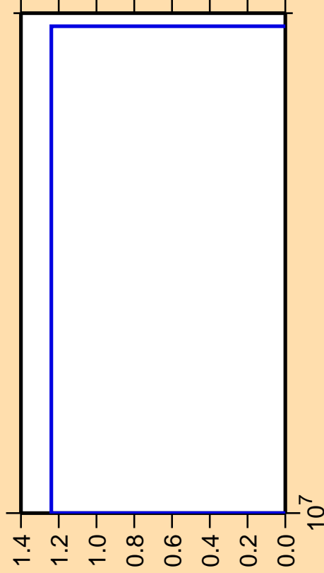
\Delta\sigma/\sigma vs. E for ^{179}\text{Re}(n,pd)
