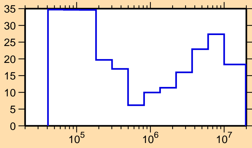
\Delta\sigma/\sigma vs. E for ^{179}\text{Re}(n,\text{el.})
