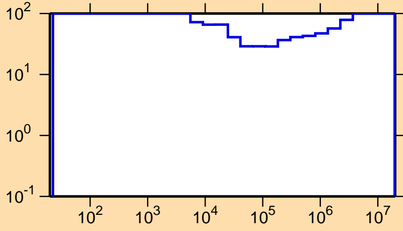
\Delta\sigma/\sigma vs. E for ^{179}\text{Re}(n,\gamma)
