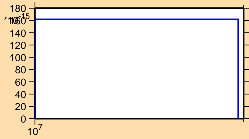
\sigma vs. E for ^{179}\text{Re}(n,pd)
