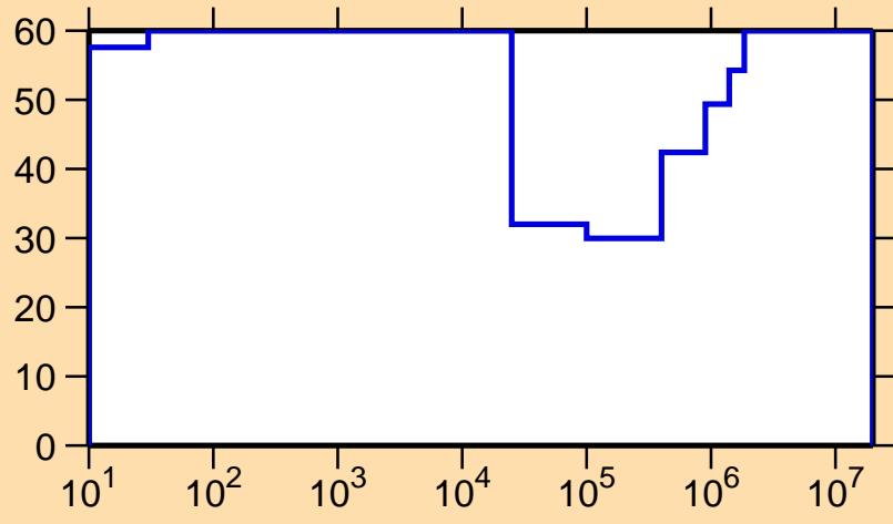
\Delta\sigma/\sigma vs. E for ^{179}\text{Re}(n,\gamma)
