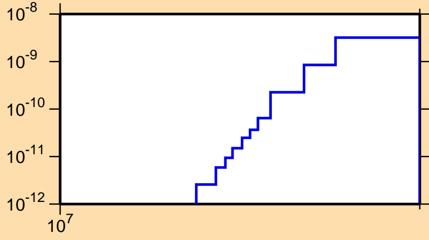
\sigma vs. E for ^{180}\text{Re}(\text{mt117})
