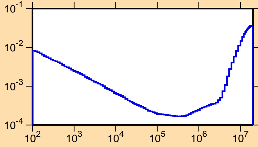
\sigma vs. E for ^{180}\text{Re}(n,p)
