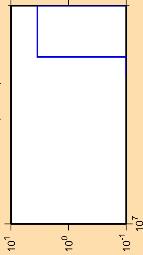
\Delta\sigma/\sigma vs. E for ^{180}\text{Re}(n,3n\alpha)
