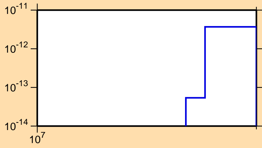
\sigma vs. E for ^{180}\text{Re}(n,pd)
