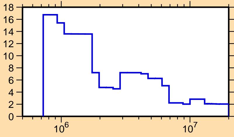
\Delta\sigma/\sigma vs. E for ^{180}\text{Re}(n,\text{tot.})
