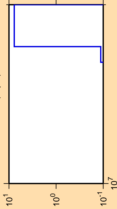
\Delta\sigma/\sigma vs. E for ^{180}\text{Re}(n,pd)
