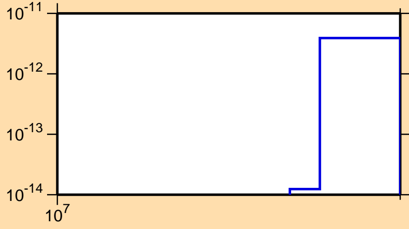
\sigma vs. E for ^{180}\text{Re}(n,3n\alpha)
