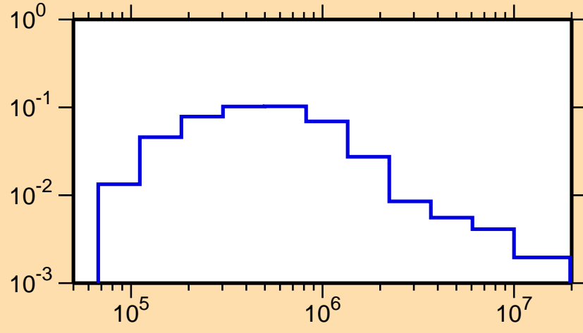
\sigma vs. E for ^{180}\text{Re}(n,n_3)
