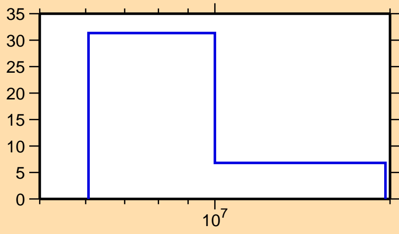
\Delta\sigma/\sigma vs. E for ^{180}\text{Re}(n,2n)
