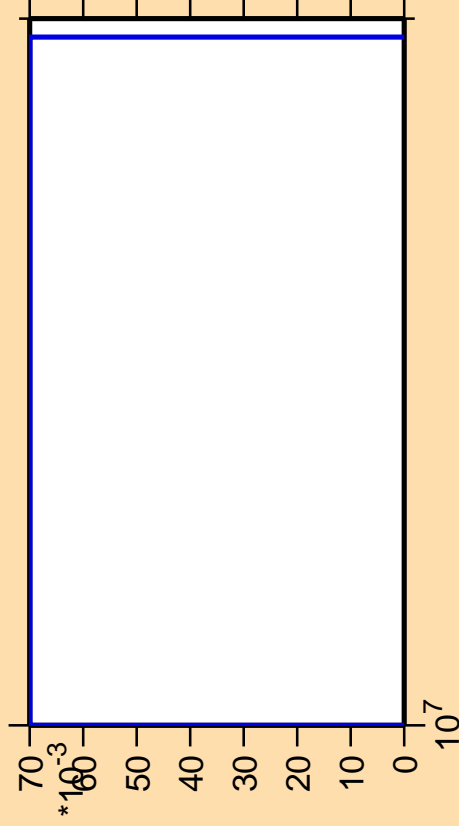
\Delta\sigma/\sigma vs. E for ^{180}\text{Re}(n,pd)
