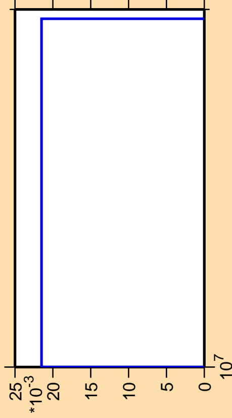
\Delta\sigma/\sigma vs. E for ^{180}\text{Re}(n,3n\alpha)
