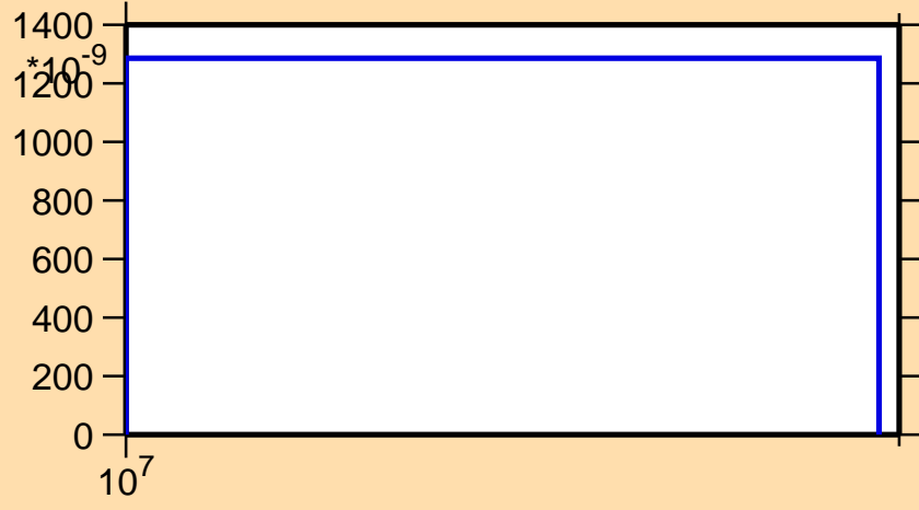
\sigma vs. E for ^{180}\text{Re}(n,nd)
