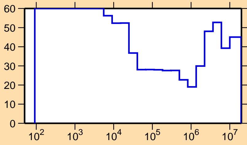
\Delta\sigma/\sigma vs. E for ^{180}\text{Re}(n,\gamma)
