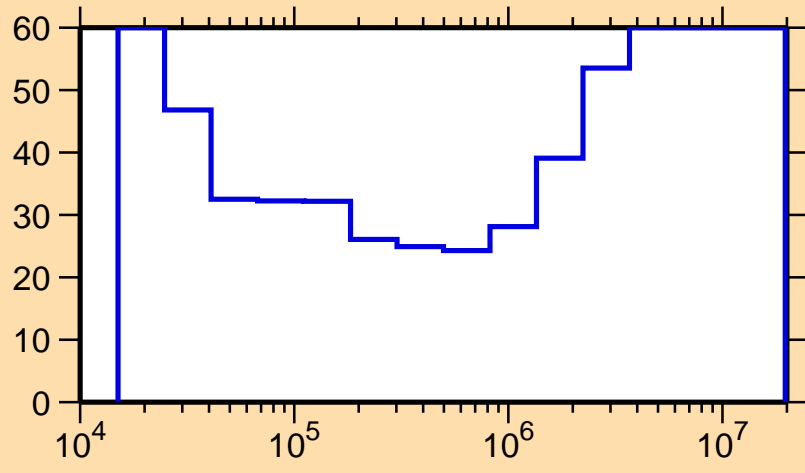
\Delta\sigma/\sigma vs. E for ^{180}\text{Re}(n,n_1)
