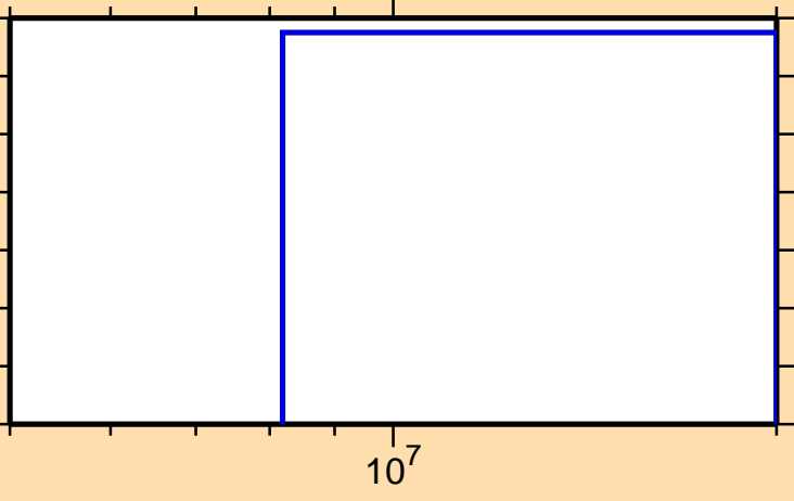
\sigma vs. E for ^{180}\text{Re}(n,3n)
