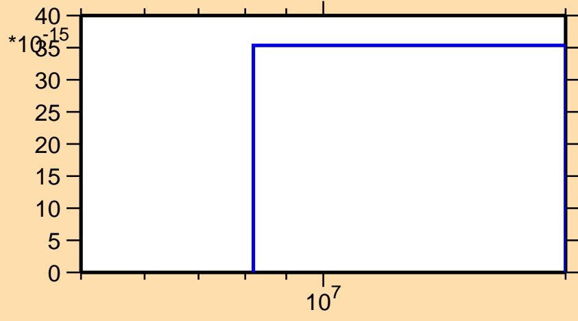
\sigma vs. E for ^{180}\text{Re}(n,3n\alpha)
