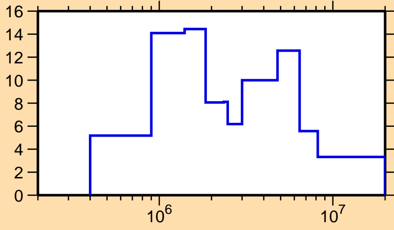
\Delta\sigma/\sigma vs. E for ^{180}\text{Re}(n, el.)
