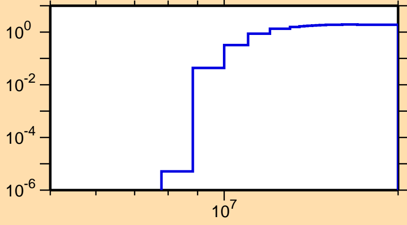
\sigma vs. E for ^{181}\text{Re}(n,2n)
