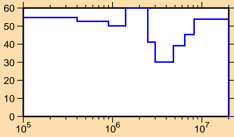
\Delta\sigma/\sigma vs. E for ^{181}\text{Re}(n,n_1)
