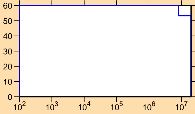
\Delta\sigma/\sigma vs. E for ^{181}\text{Re}(n,p)
