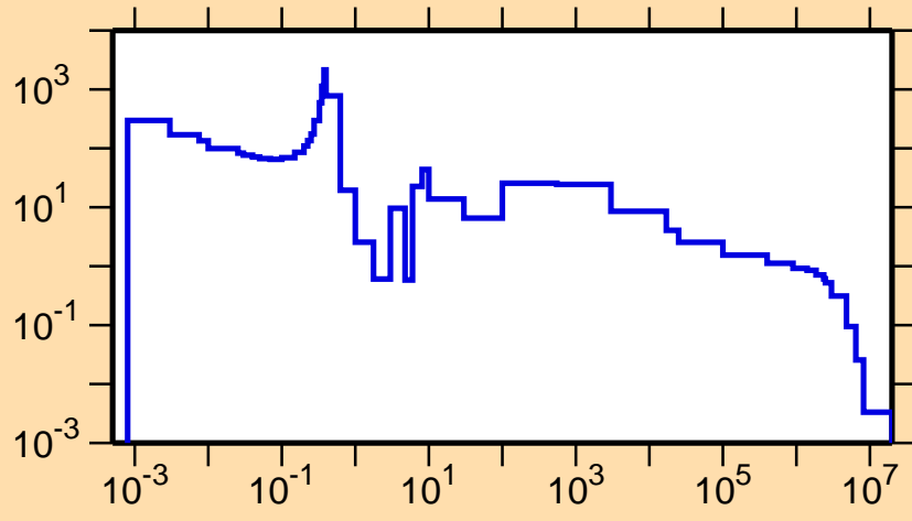
\sigma vs. E for ^{181}\text{Re}(n,\gamma)
