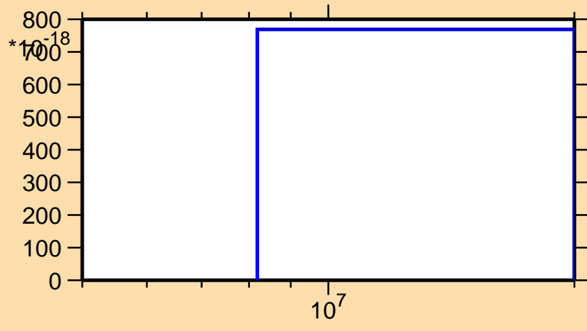
\sigma vs. E for ^{181}\text{Re}(n,\text{pd})
