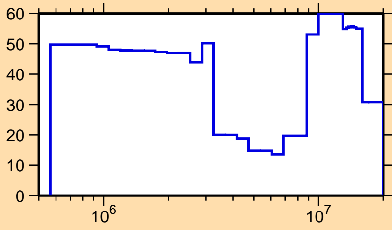
\Delta\sigma/\sigma vs. E for ^{182}\text{Re}(n,n\text{cont.})
