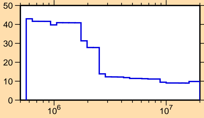
\Delta\sigma/\sigma vs. E for ^{182}\text{Re}(n,n\text{onel.})
