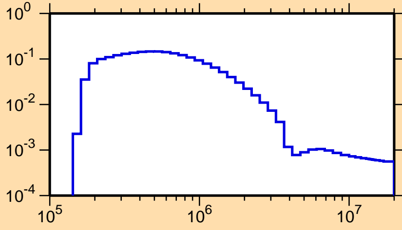
\sigma vs. E for ^{182}\text{Re}(n,n_1)
