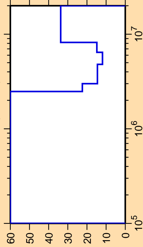
\Delta\sigma/\sigma vs. E for ^{182}\text{Re}(n,\text{inel.})
