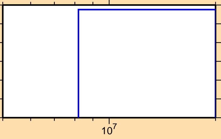
\sigma vs. E for ^{182}\text{Re}(n,\text{nd})
