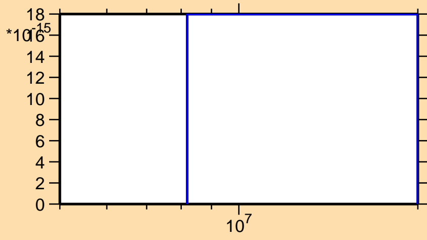
\sigma vs. E for ^{182}\text{Re}(n,3n\alpha)
