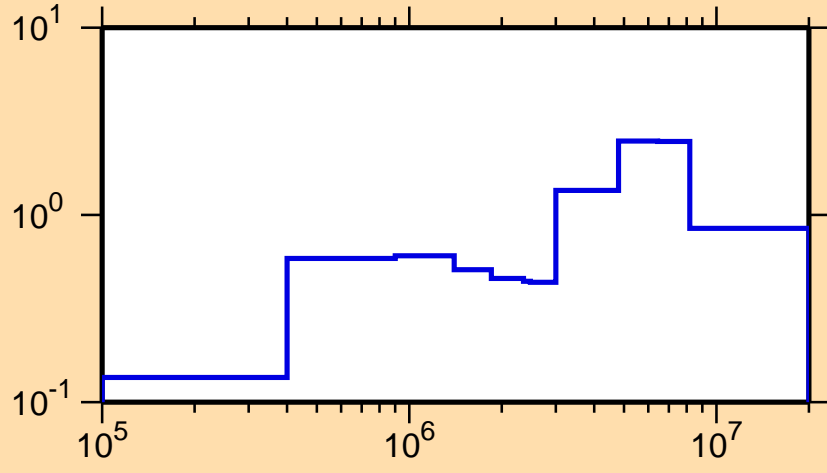
\sigma vs. E for ^{182}\text{Re}(n,\text{inel.})
