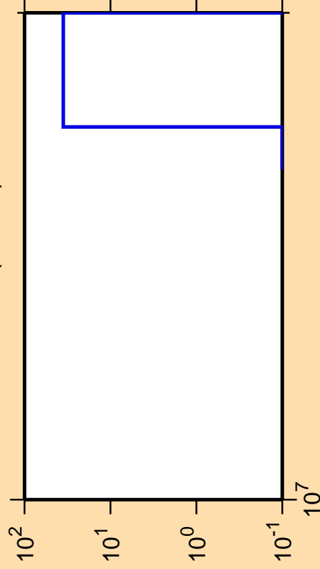
\Delta\sigma/\sigma vs. E for ^{182}\text{Re}(n,3n\alpha)
