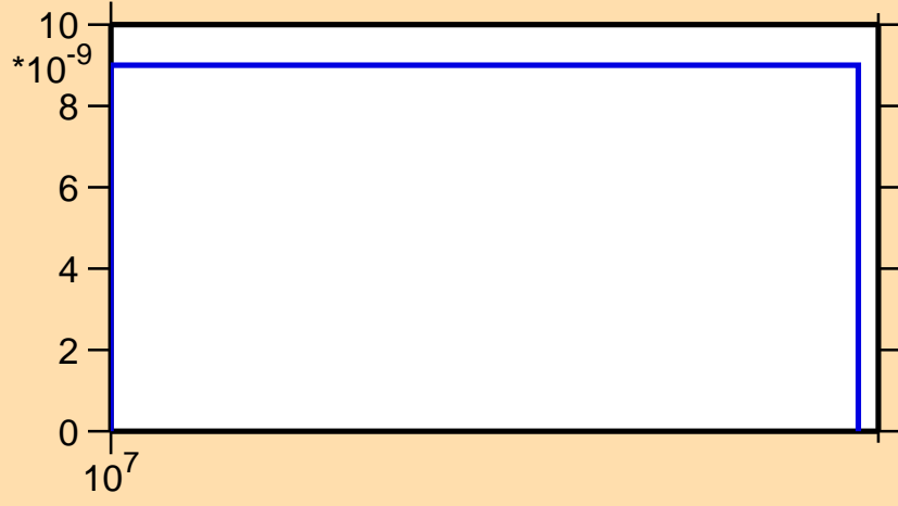
\sigma vs. E for ^{182}\text{Re}(n,nt)
