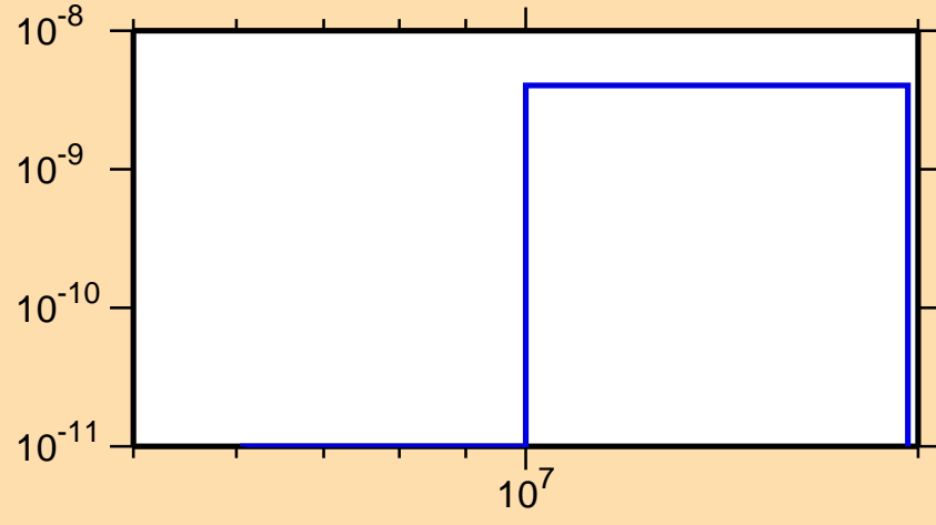
\sigma vs. E for ^{182}\text{Re}(n,p\alpha)
