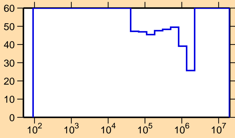
\Delta\sigma/\sigma vs. E for ^{182}\text{Re}(n,\gamma)
