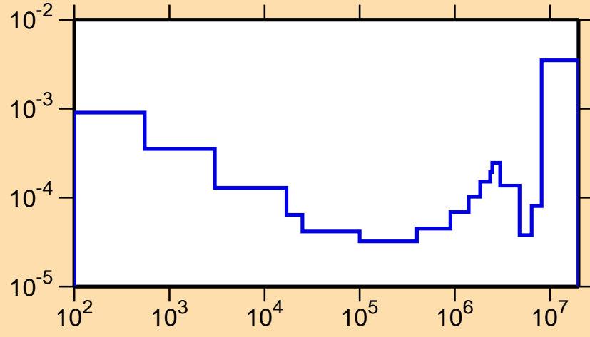
\sigma vs. E for ^{182}\text{Re}(n,\alpha)
