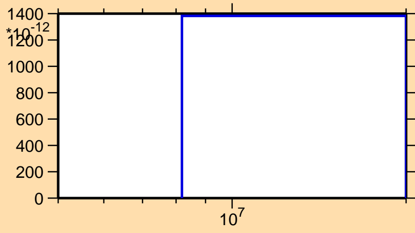
\sigma vs. E for ^{182}\text{Re}(n,\text{He3})
