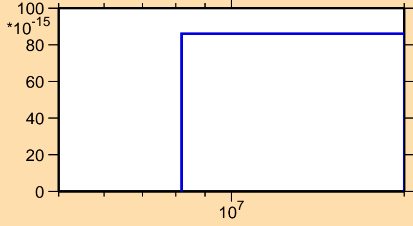
\sigma vs. E for ^{182}\text{Re}(n,3n\alpha)
