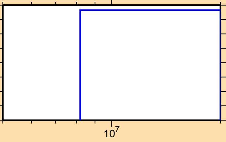
\sigma vs. E for ^{182}\text{Re}(n,3n)
