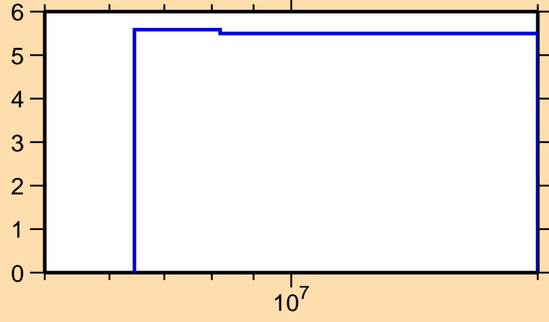
\Delta\sigma/\sigma vs. E for ^{182}\text{Re}(n,\text{el.})
