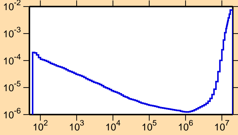
\sigma vs. E for ^{184}\text{Re}(n,\alpha)
