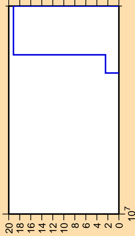
\Delta\sigma/\sigma vs. E for ^{184}\text{Re}(\text{mt117})
