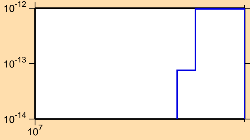
\sigma vs. E for ^{184}\text{Re}(\text{mt } 45)
