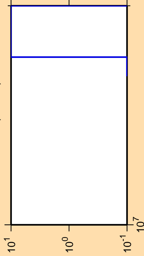
\Delta\sigma/\sigma vs. E for ^{184}\text{Re}(n,3n\alpha)
