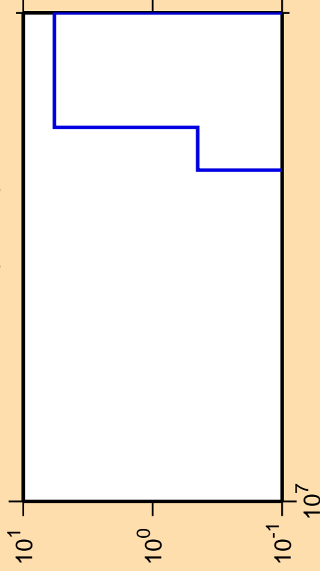
\Delta\sigma/\sigma vs. E for ^{184}\text{Re}(\text{mt } 45)
