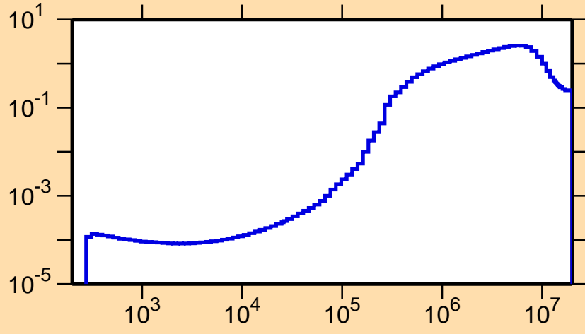
\sigma vs. E for ^{184}\text{Re}(n,\text{inel.})
