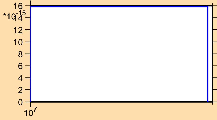
\sigma vs. E for ^{184}\text{Re}(\text{mt } 45)
