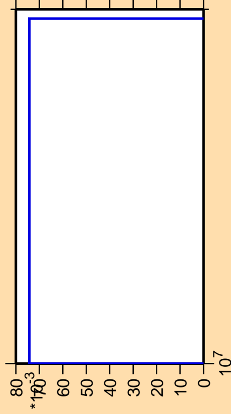
\Delta\sigma/\sigma vs. E for ^{184}\text{Re}(\text{mt } 45)
