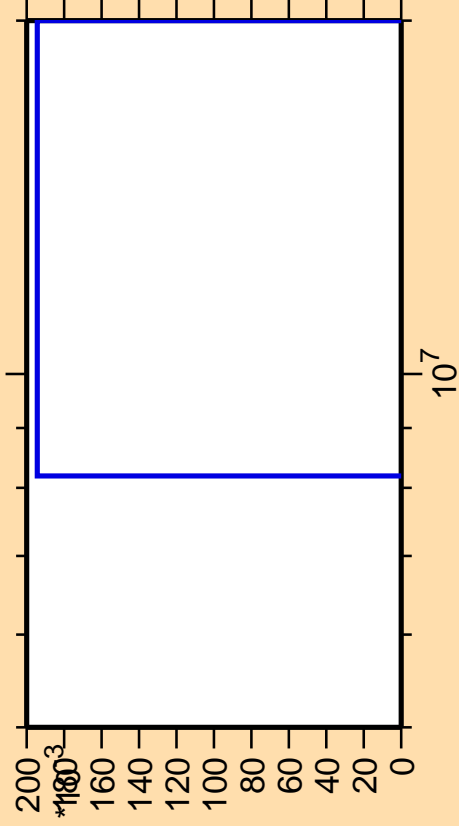
\Delta\sigma/\sigma vs. E for ^{184}\text{Re}(n,3n\alpha)
