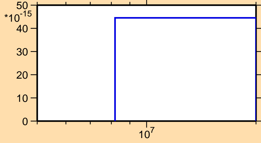
\sigma vs. E for ^{184}\text{Re}(\text{mt117})
