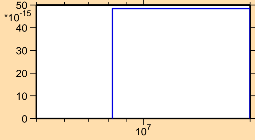
\sigma vs. E for ^{184}\text{Re}(n,3n\alpha)
