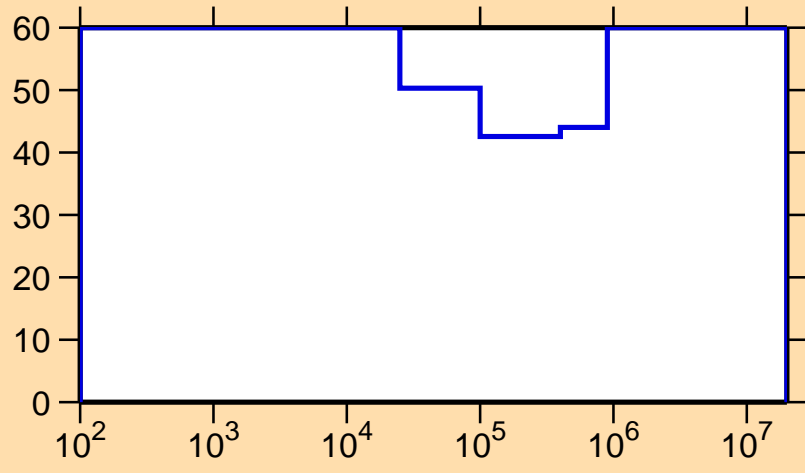
\Delta\sigma/\sigma vs. E for ^{184}\text{Re}(n,\gamma)
