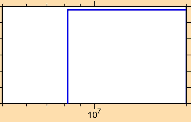
\sigma vs. E for ^{184}\text{Re}(n,\text{nd})
