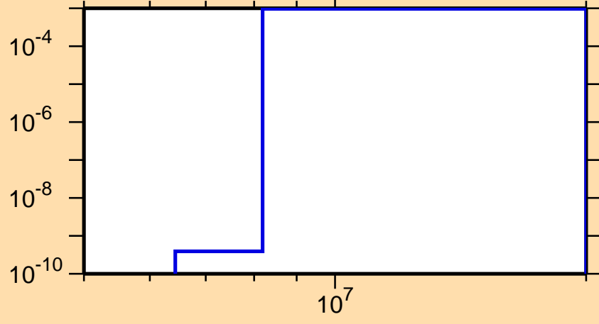
\sigma vs. E for ^{184}\text{Re}(n,d)
