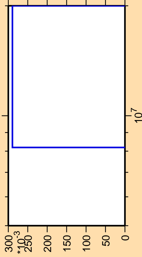
\Delta\sigma/\sigma vs. E for ^{184}\text{Re}(\text{mt117})
