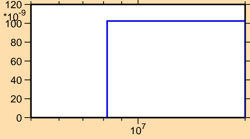
\sigma vs. E for ^{184}\text{Re}(n,2np)
