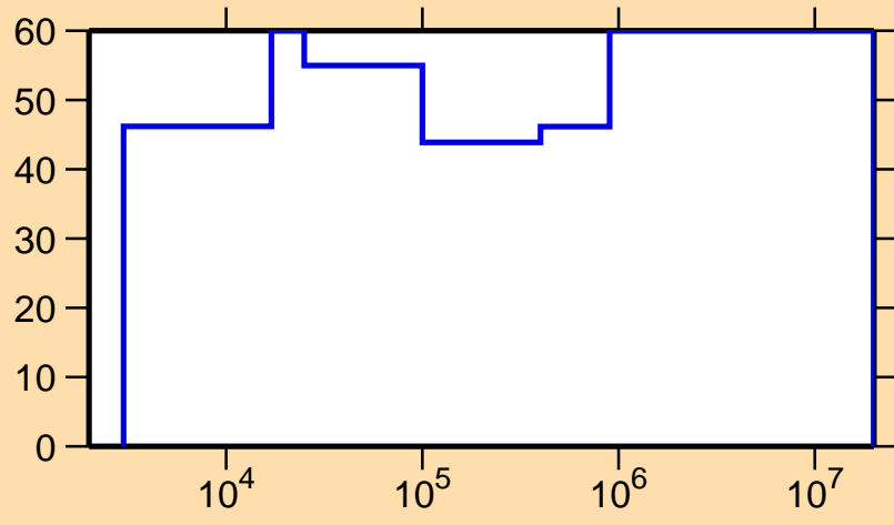
\Delta\sigma/\sigma vs. E for ^{184}\text{Re}(n,n_1)
