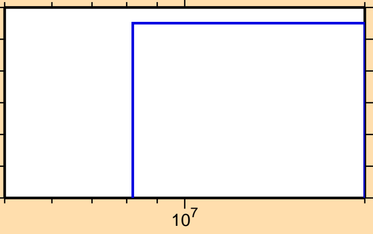
\sigma vs. E for ^{184}\text{Re}(n,3n)
