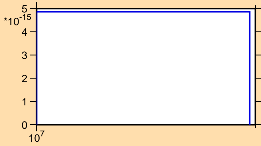
\sigma vs. E for ^{185}\text{Re}(\text{mt } 45)
