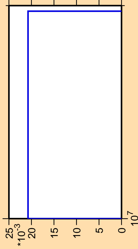
\Delta\sigma/\sigma vs. E for ^{185}\text{Re}(\text{mt } 45)
