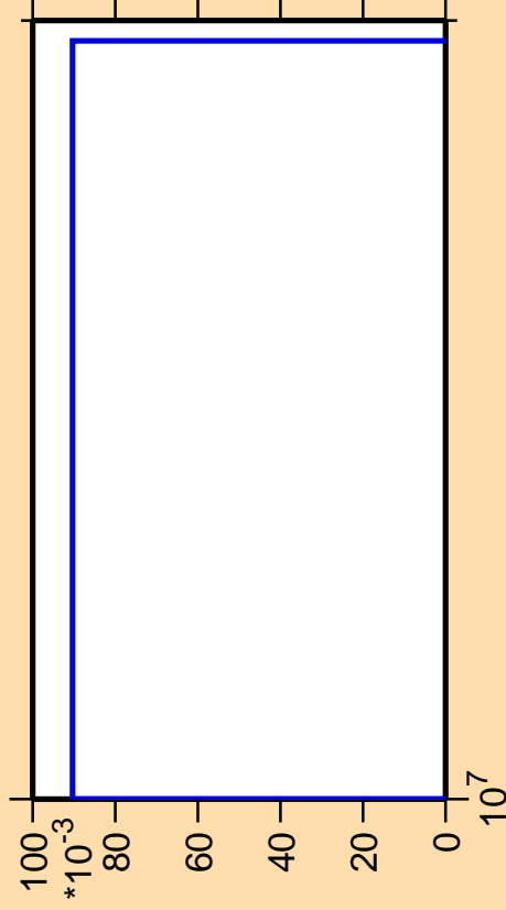
\Delta\sigma/\sigma vs. E for ^{185}\text{Re}(n,3n\alpha)
