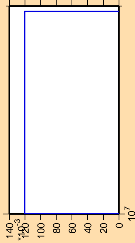
\Delta\sigma/\sigma vs. E for ^{185}\text{Re}(\text{mt117})
