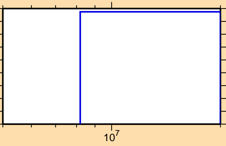
\sigma vs. E for ^{185}\text{Re}(\text{mt117})
