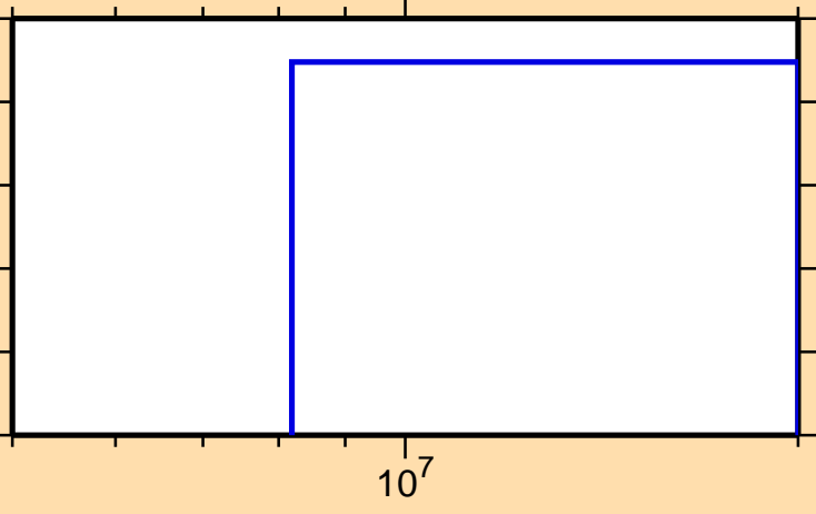
\sigma vs. E for ^{185}\text{Re}(n,p\alpha)
