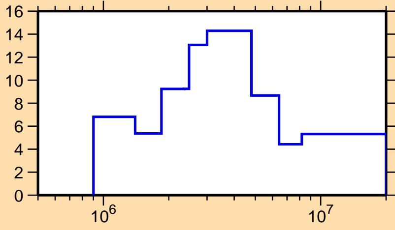
\Delta\sigma/\sigma vs. E for ^{185}\text{Re}(n, el.)
