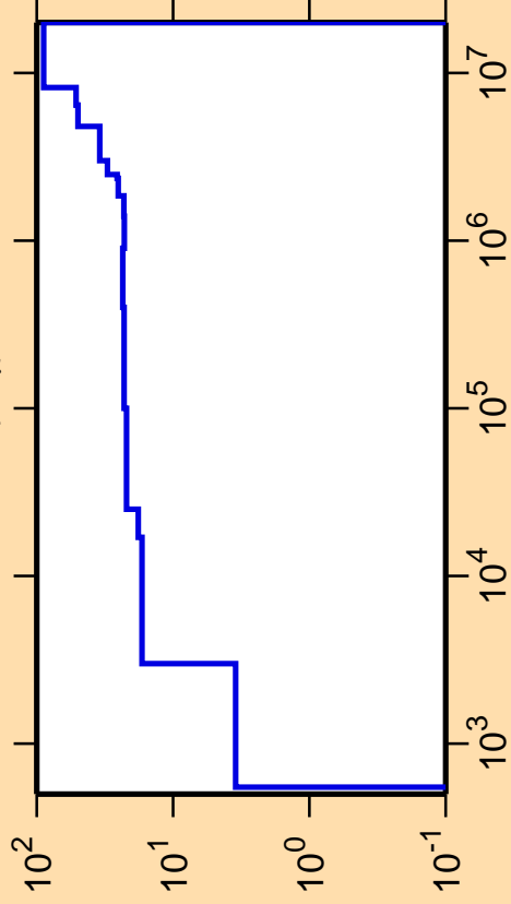
\Delta\sigma/\sigma vs. E for ^{185}\text{Re}(n,\gamma)
