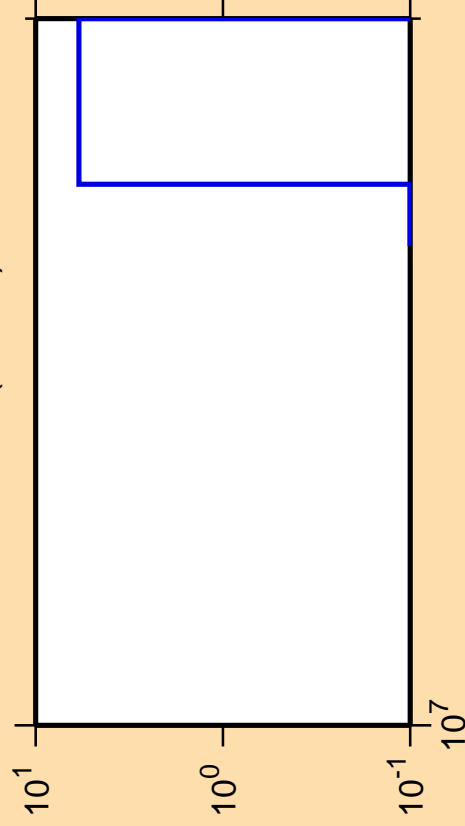
\Delta\sigma/\sigma vs. E for ^{186}\text{Re}(n,3n\alpha)
