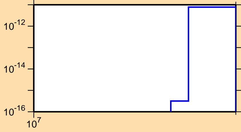
\sigma vs. E for ^{186}\text{Re}(n,3n\alpha)
