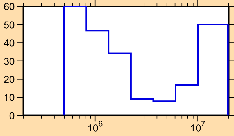
\Delta\sigma/\sigma vs. E for ^{186}\text{Re}(n,n\text{cont.})
