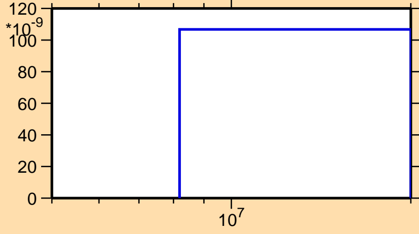
\sigma vs. E for ^{186}\text{Re}(n,2np)
