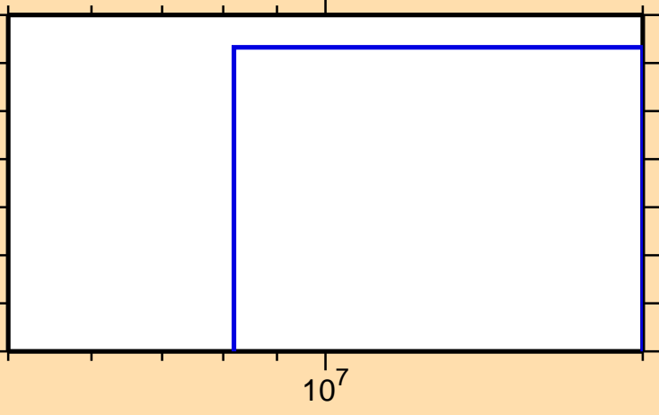
\sigma vs. E for ^{186}\text{Re}(n,3n\alpha)
