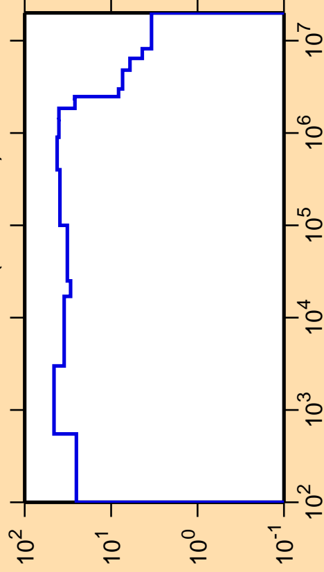
\Delta\sigma/\sigma vs. E for ^{186}\text{Re}(n,\text{nonel.})
