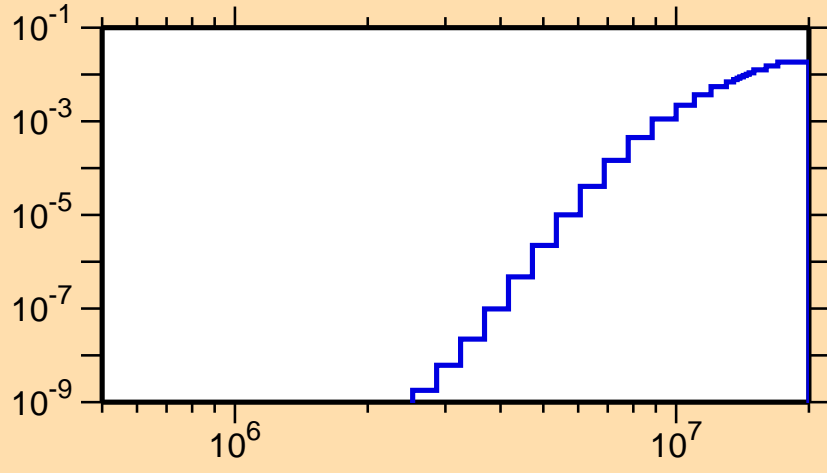
\sigma vs. E for ^{186}\text{Re}(n,p)
