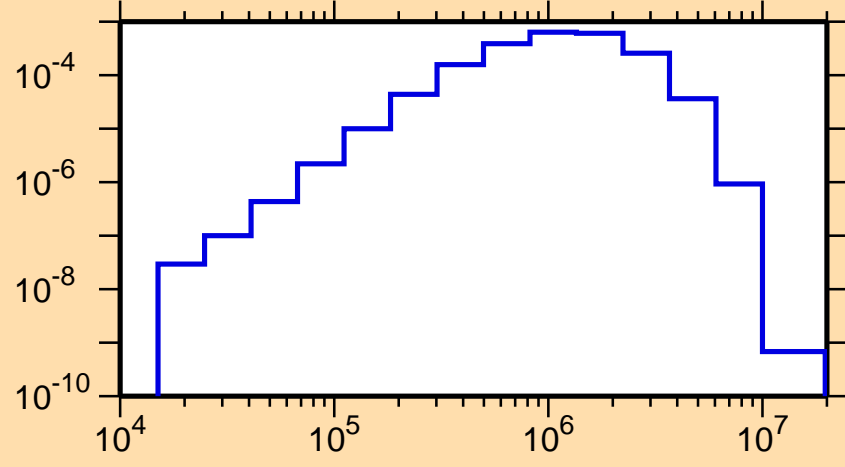
\sigma vs. E for ^{186}\text{Re}(n,n_3)
