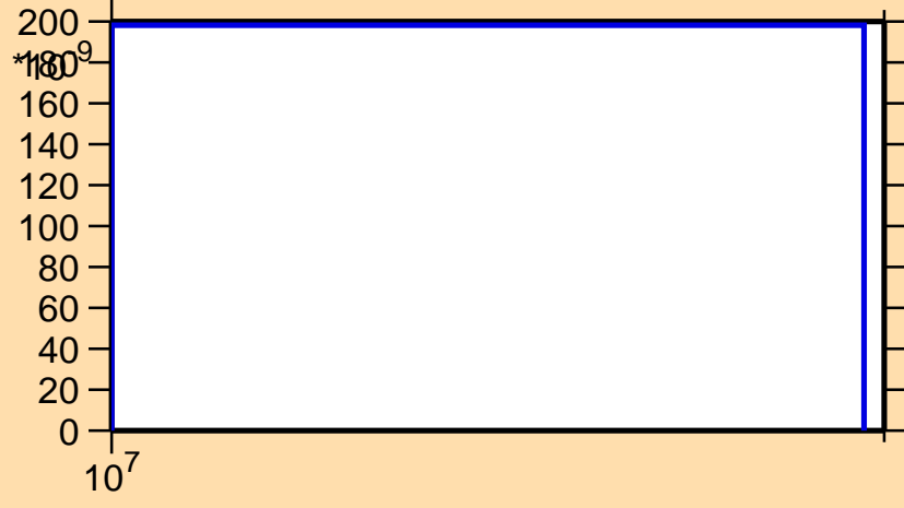
\sigma vs. E for ^{186}\text{Re}(n,\text{nd})
