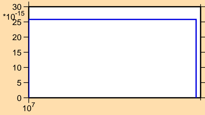
\sigma vs. E for ^{186}\text{Re}(n,3n\alpha)
