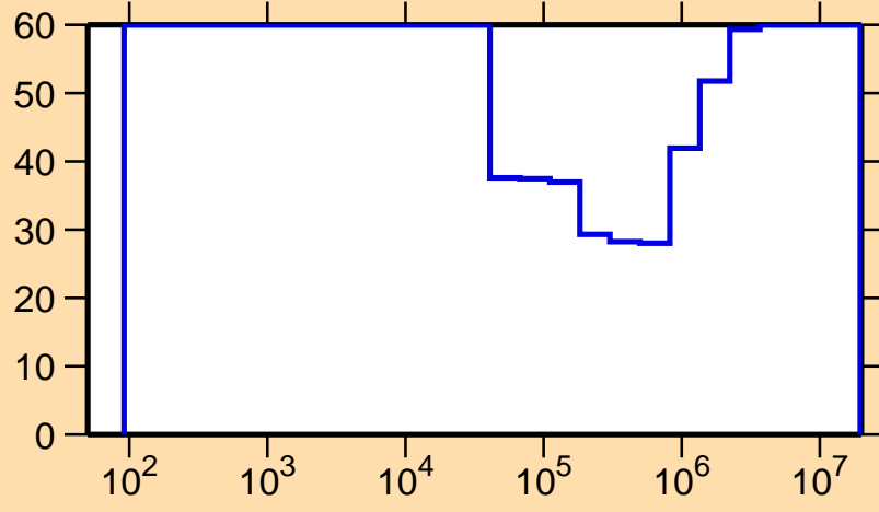
\Delta\sigma/\sigma vs. E for ^{186}\text{Re}(n,\gamma)
