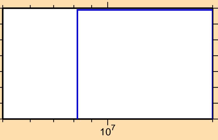
\sigma vs. E for ^{186}\text{Re}(n,3n)
