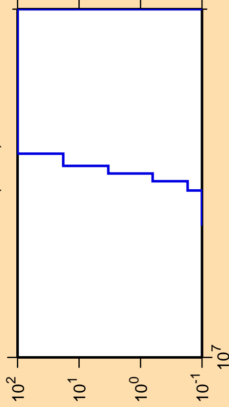
\Delta\sigma/\sigma vs. E for ^{187}\text{Re}(n,nd)
