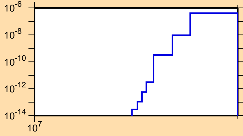
\sigma vs. E for ^{187}\text{Re}(n,nd)
