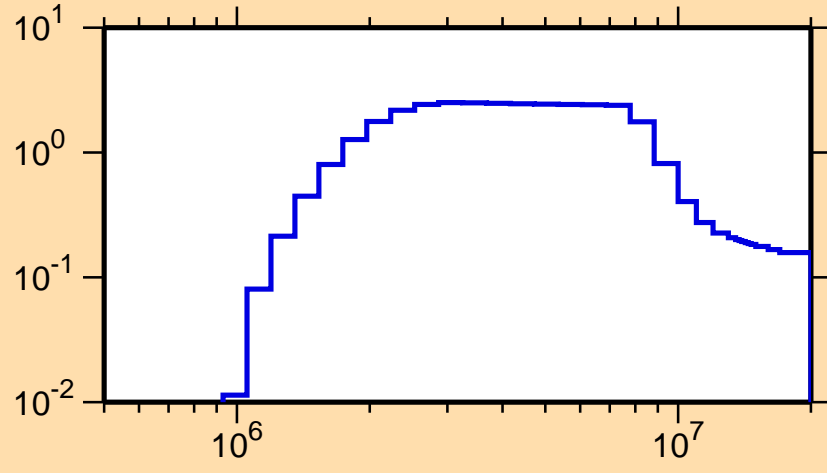
\sigma vs. E for ^{187}\text{Re}(n,n\text{cont.})
