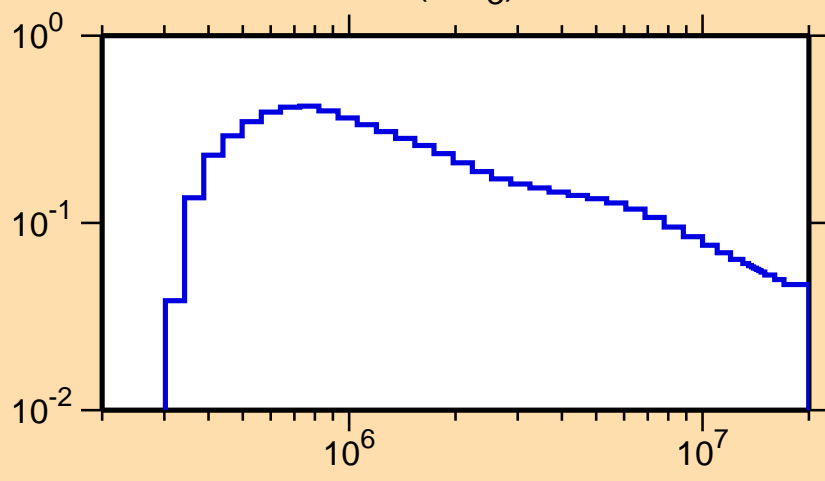
\sigma vs. E for ^{187}\text{Re}(n,n_3)
