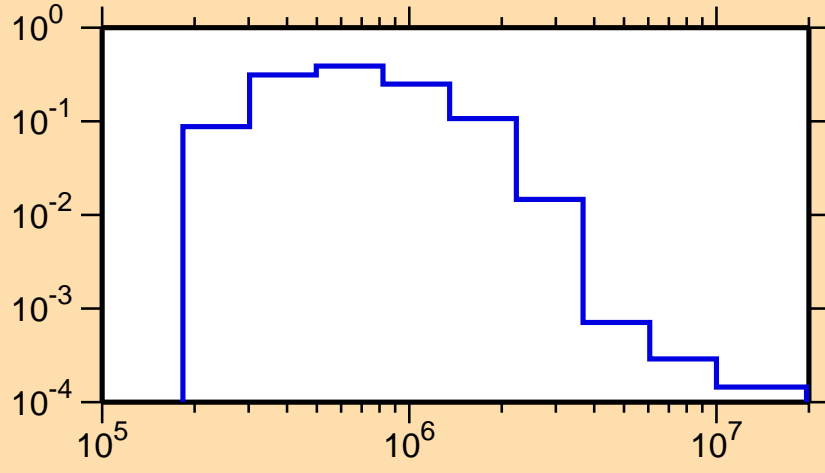
\sigma vs. E for ^{187}\text{Re}(n,n_2)
