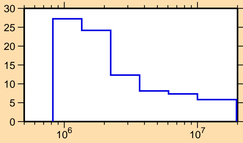
\Delta\sigma/\sigma vs. E for ^{187}\text{Re}(n,n\text{onel.})
