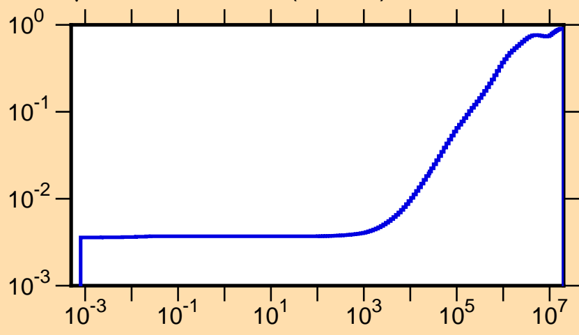
\mu vs. E for ^{188}\text{Re}(\text{mt251})
