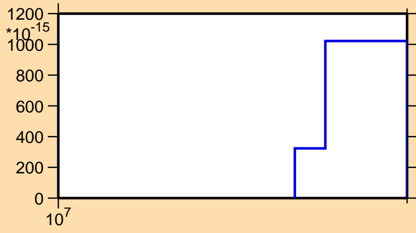
\sigma vs. E for ^{188}\text{Re}(n,p\alpha)
