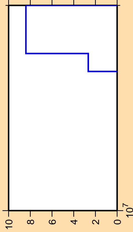
\Delta\sigma/\sigma vs. E for ^{188}\text{Re}(n,p\alpha)
