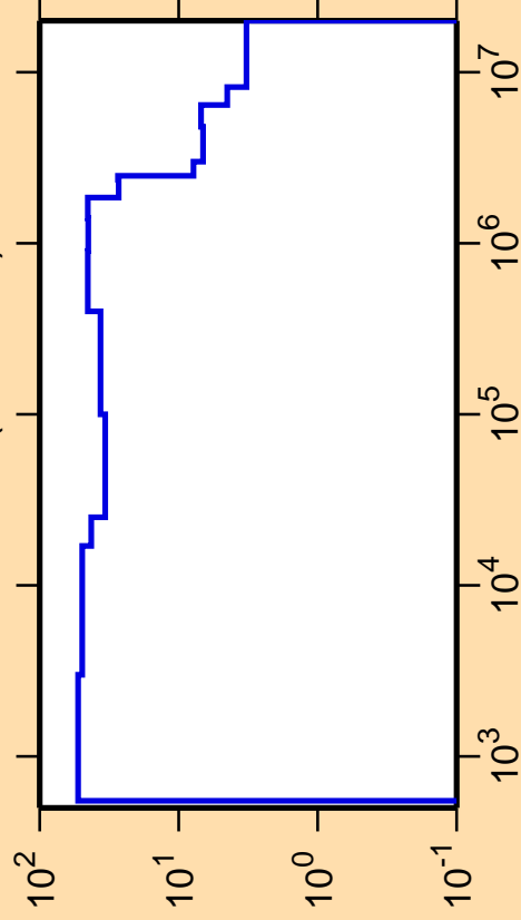
\Delta\sigma/\sigma vs. E for ^{188}\text{Re}(n,\text{nonel.})
