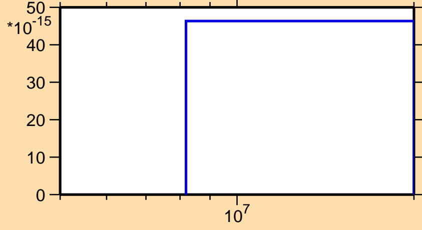
\sigma vs. E for ^{188}\text{Re}(n,p\alpha)
