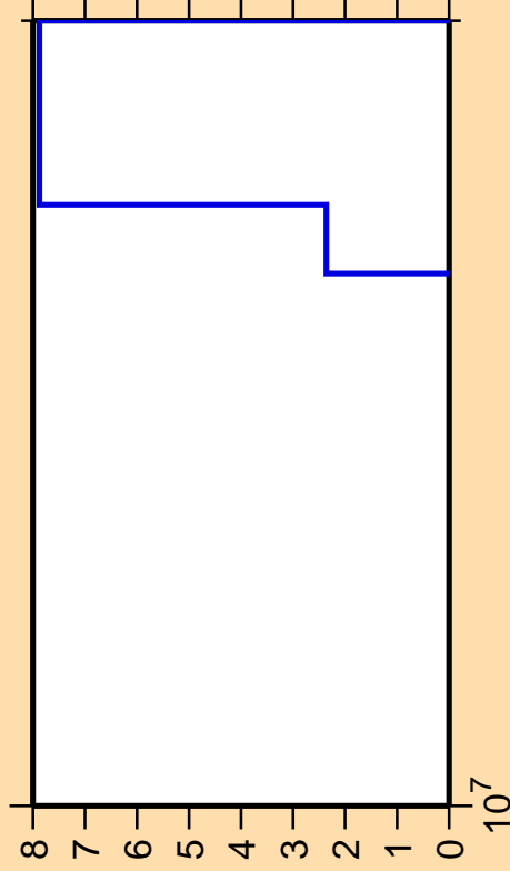
\Delta\sigma/\sigma vs. E for ^{188}\text{Re}(n,p\alpha)
